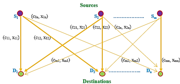
Fig. 1. Simplified form of the transportation problem.
