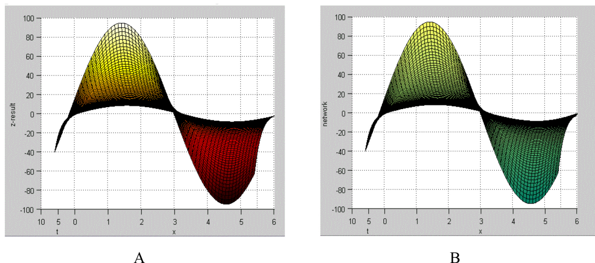
Fig. 4. A- The exact solution, B- The neural network result.
