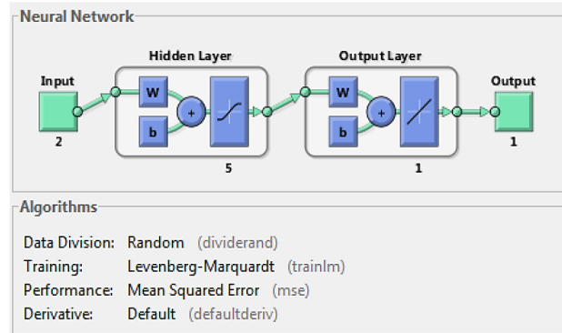
Fig. 2. Structure of ANN in Matlab.
