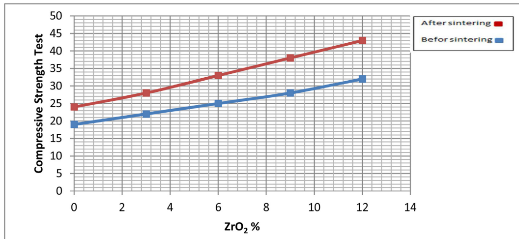
Figure 2. The relationship of compressive strength and zirconia nanoparticles before and after heat treatment.
