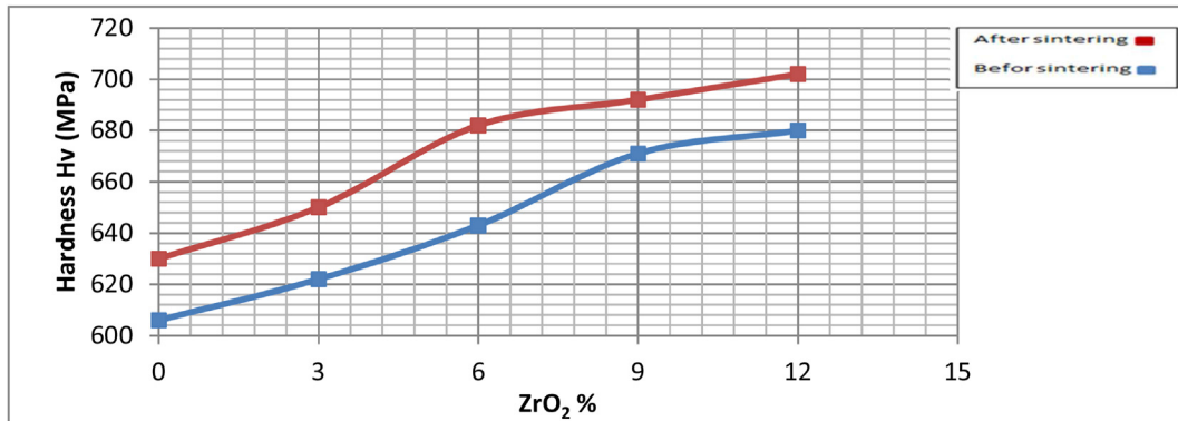
Figure 4. Clearly shows the positive relationship between zirconia nanoparticles and Vickers micro hardness before and after heat treatment.
