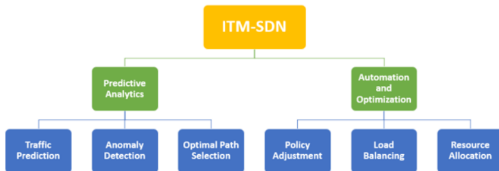
Figure 3. Main methods of intelligent traffic management.
