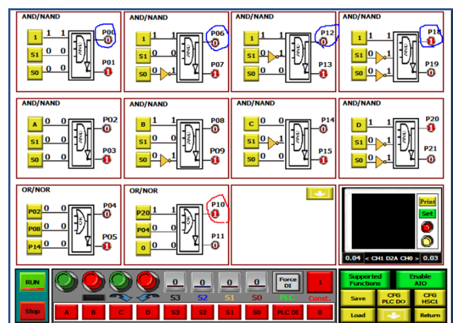
Fig. 16. Decoder and multiplexer circuits
