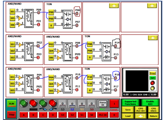
Fig. 6. Three sources changeover switch control
