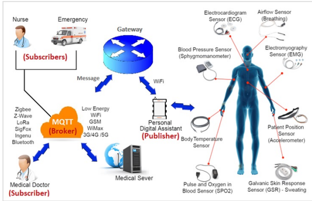
Fig. 2. MQTT deployment and subscription model for IoT sensors.
