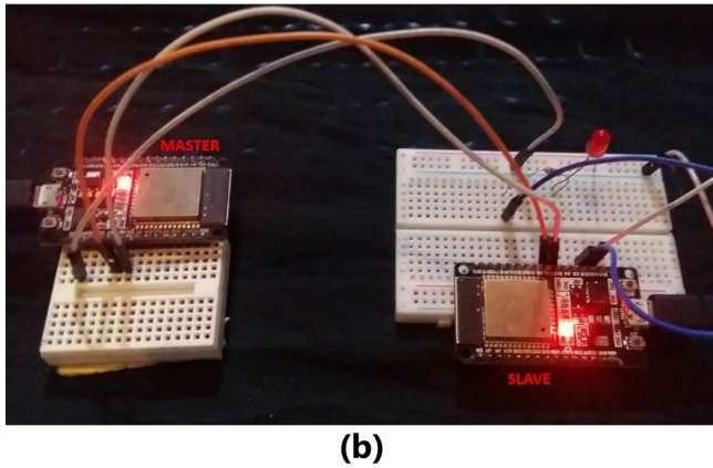
Fig. 7. UART connection of two ESP32 controllers: (a) Schematic diagram. (b) Practical circuit.
