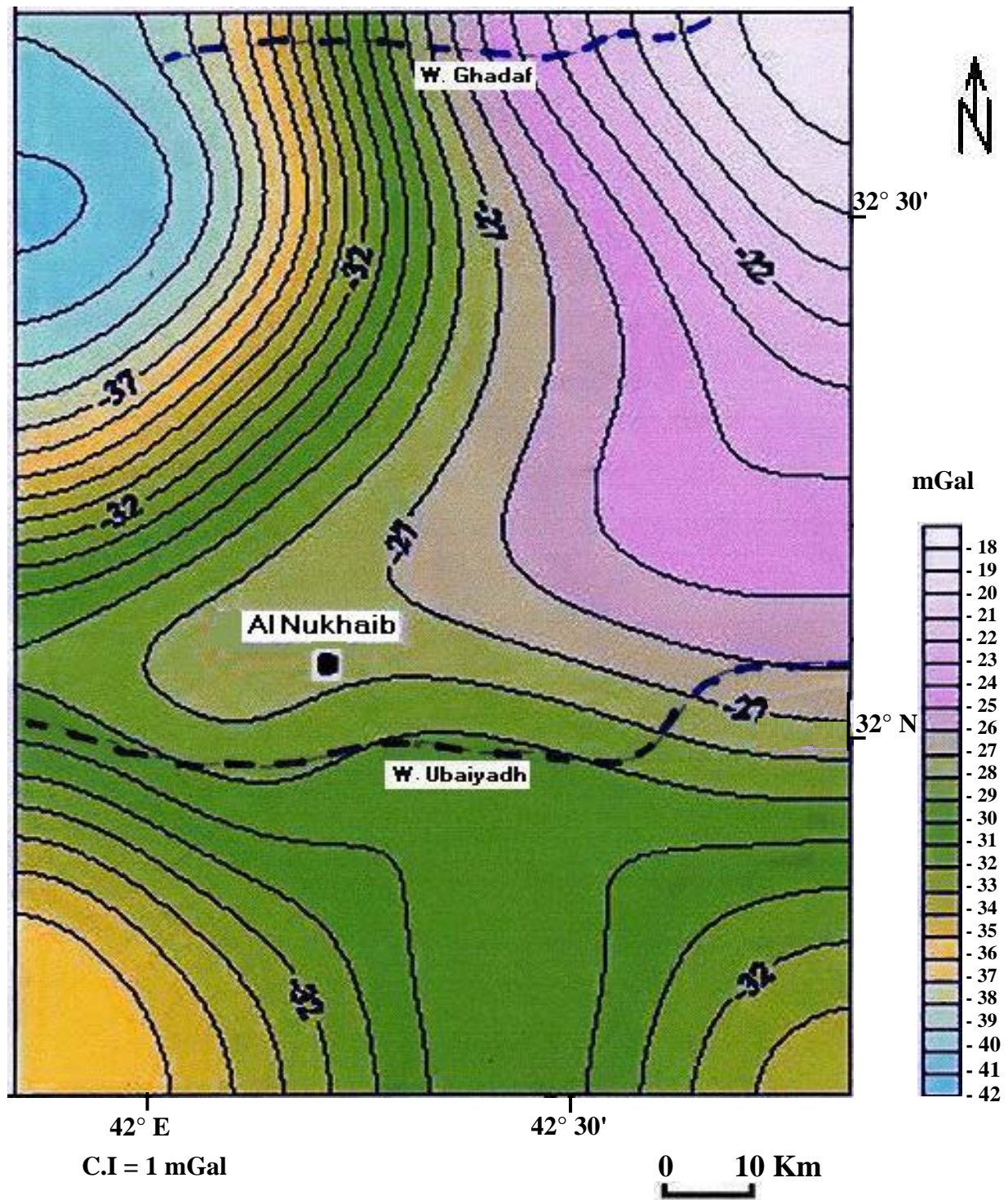
Fig.5: The regional gravity map of the study area
