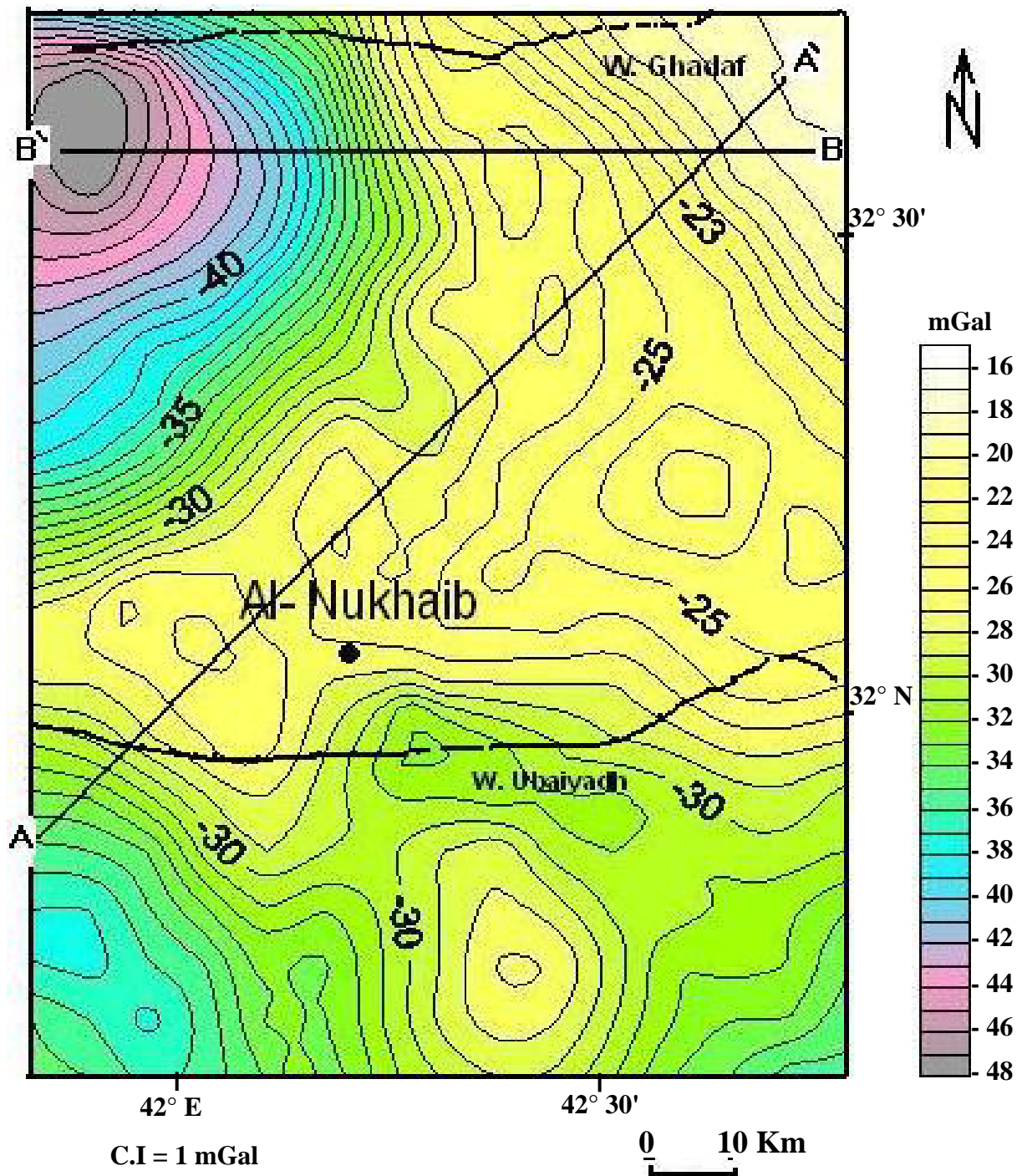
Fig.4: The observed Bouguer anomaly map (after Al-Kadhimi, 1996)
