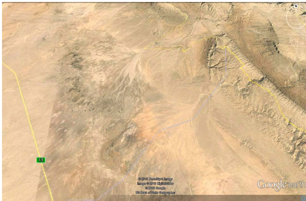
Fig.13: Google Earth image of Multi Stages Alluvial Fan in Zurbatiya vicinity, note the tone differences in different stages, as well in different parts
