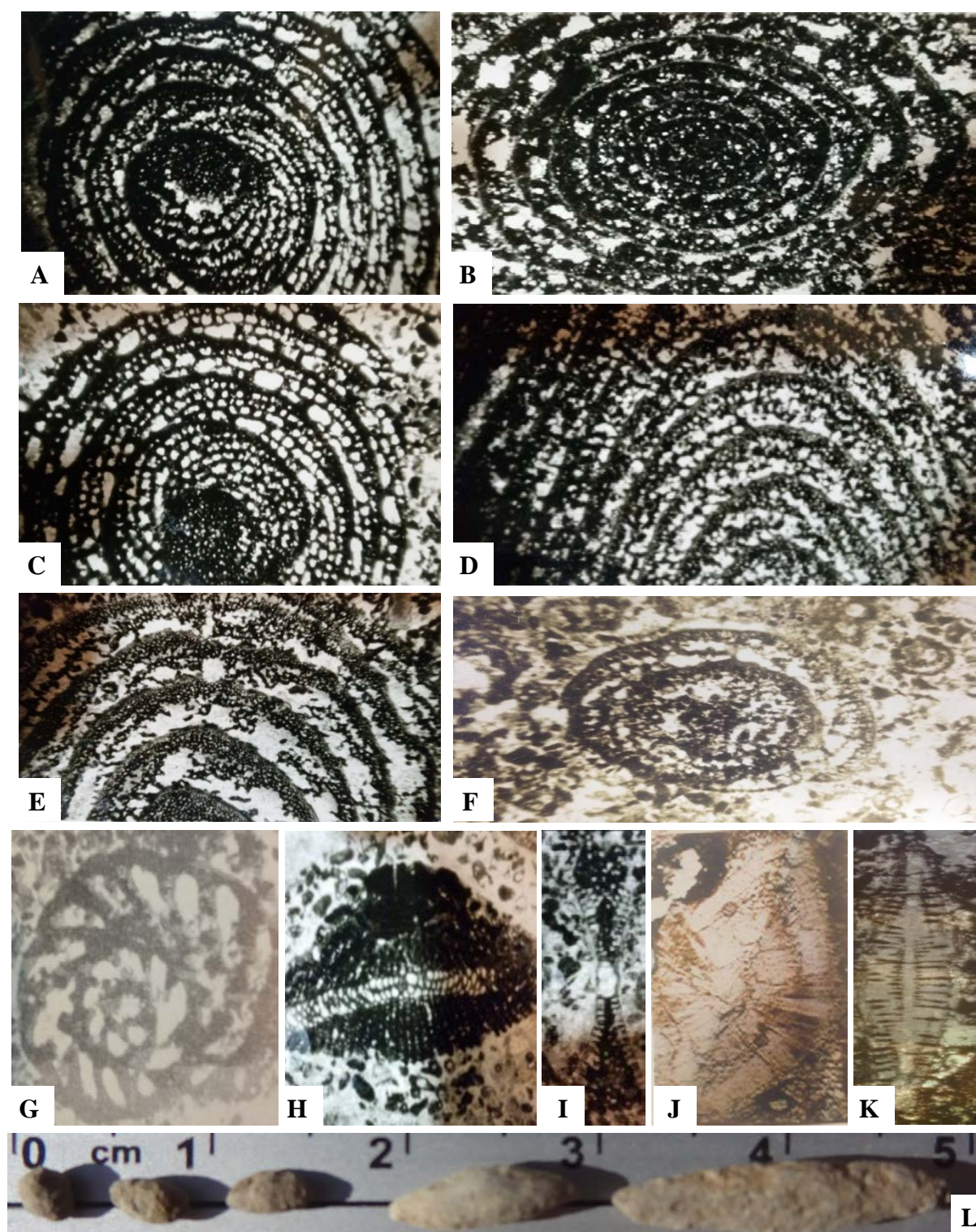
Fig.7: A and B) Loftusia elongata Coxi, equatorial view, X10. C and D) Loftusia persica Brady, equatorial and longitudinal view, X10. E) Loftusia morgani Douville, longitudinal view, X10. F) Loftusia minor Cox, equatorial view, X10. G) Loftusia coxi Henson, equatorial view, X10. H) Orbiotoides media (d' Archinc), X25. I) Omphalocyclus macroporus (Lamarck), X25. J) Fissoelphidium operculiferum Smout, X40. K) Lepidorbitoides socialis (Leymerie), X20. L) Complete form of Lofusia minor , L. Coxi , L. morgani , L. elongate , and L. Persica (all Figures from Maukaba section)
