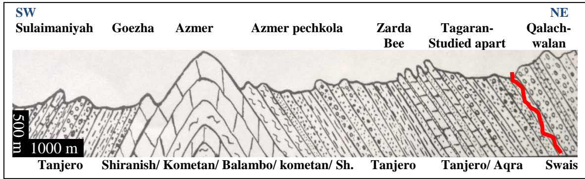
Fig.2: General geological section along Sulaimaniyah – Chwarta main road. (Oldest, Balambo fn., Kometan fn., Shiranish fn., Tanjero fn., Aqra fn., and Swais Group, Youngest)
