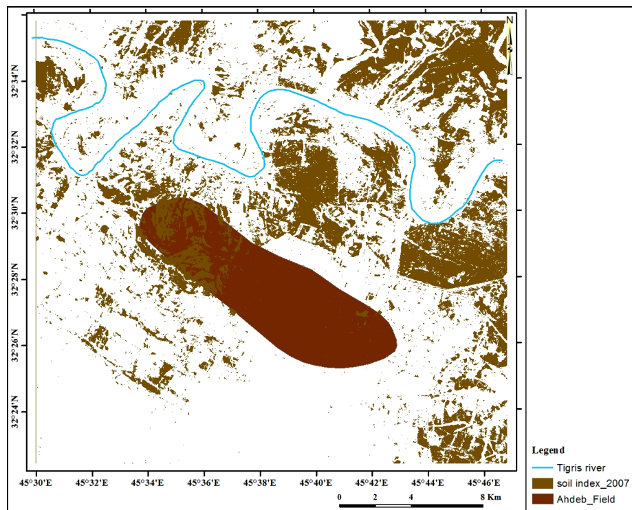
Fig.7: The Soil Index in 642 RGB for TM 2007 image
