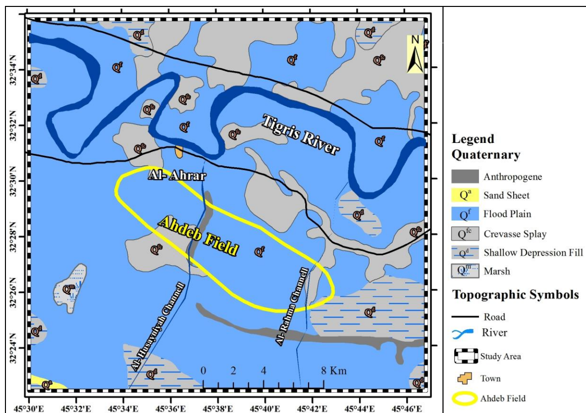
Fig.2: Geological map of the study area (after Barwary and Yacoub, 1992)
