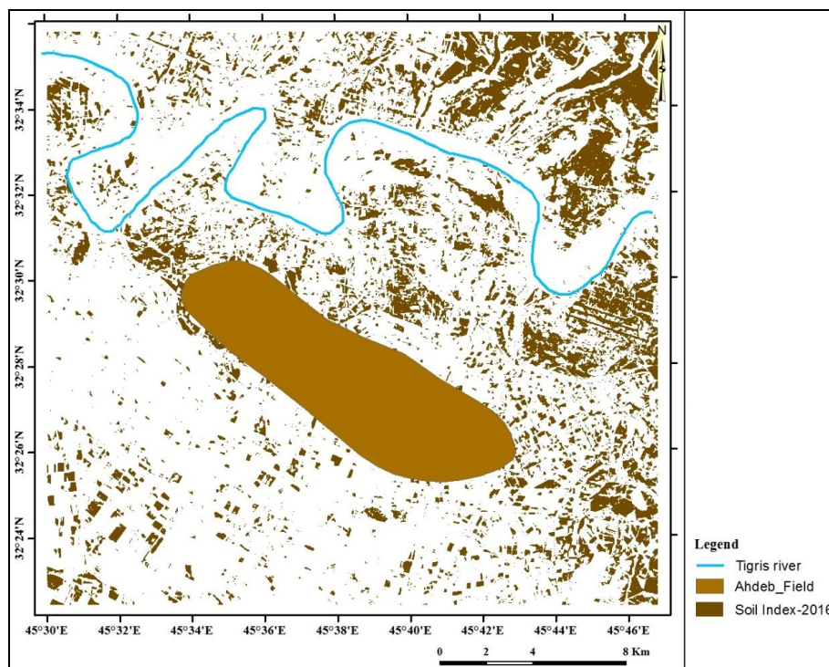
Fig.8: The Soil Index in 753 RGB for Landsat 8 OLI 2016 image
