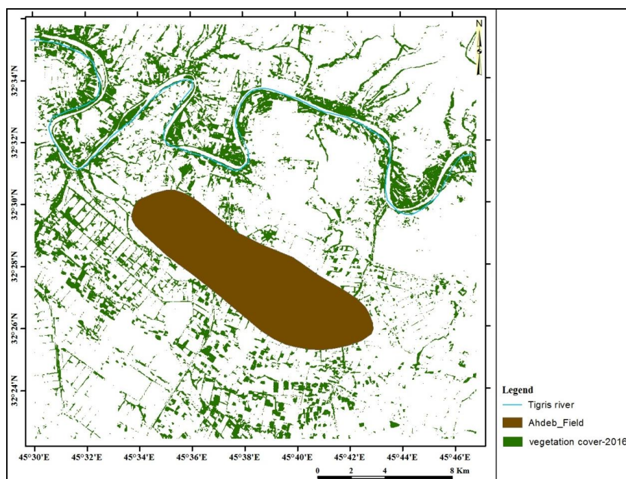
Fig.4: Vegetation cover in 753 RGB for Landsat 8 OLI 2016 image
