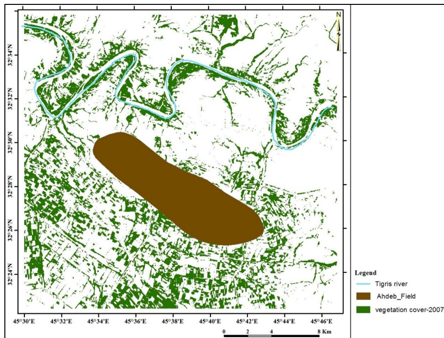
Fig.3: Vegetation cover in 642 RGB for TM 2007 image
