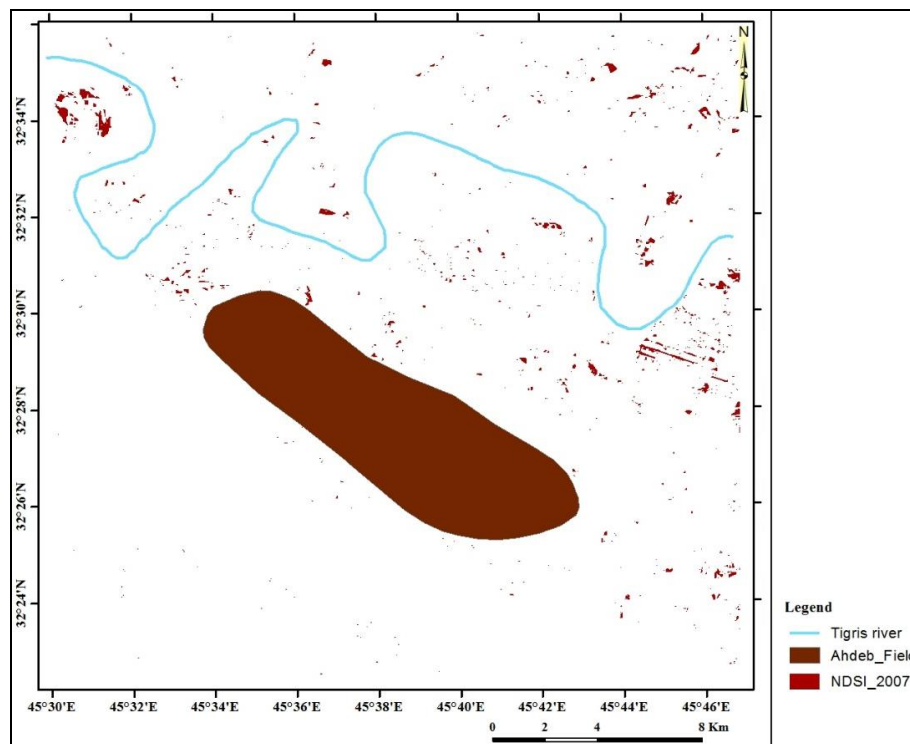
Fig.5: The NDSI in 642 RGB for TM 2007 image
