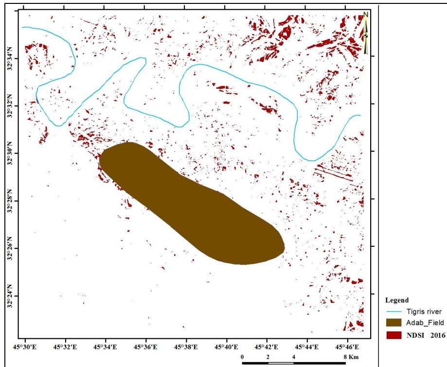
Fig.6: The NDSI in 753 RGB for Landsat 8 image
