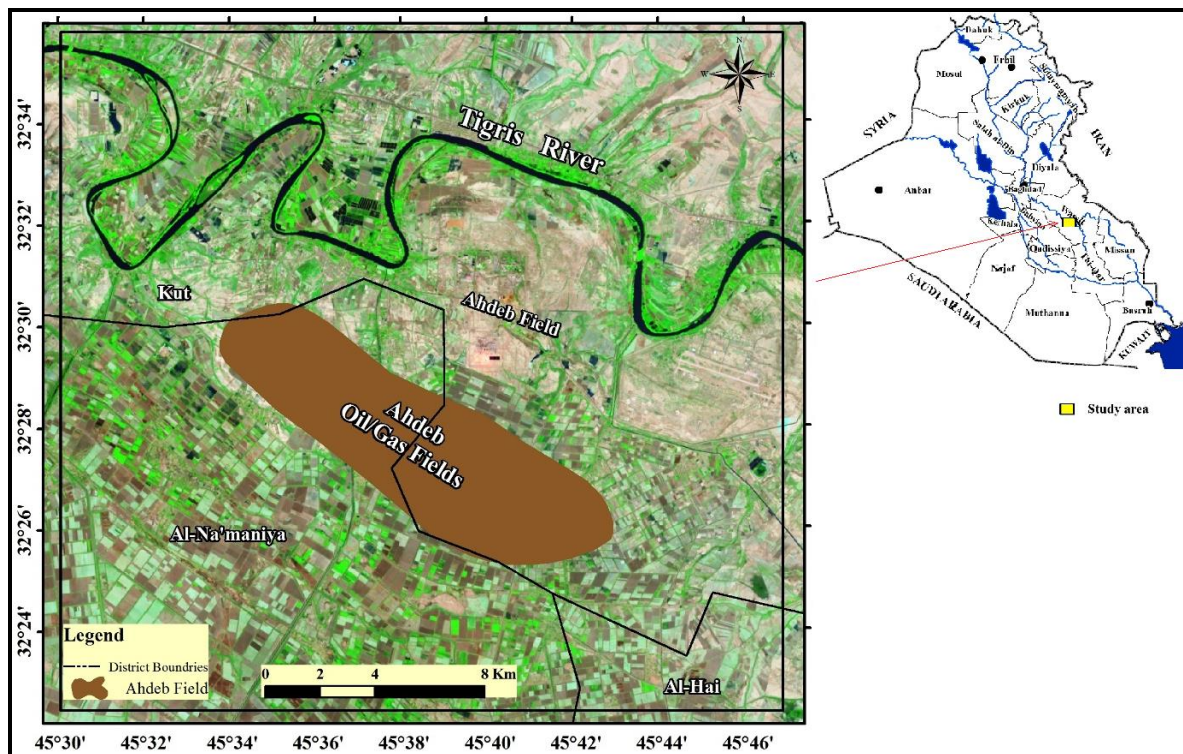
Fig.1: Location map of the study area showing Al Ahdeb oil field in 753 RGB based on Landsat 8 image
