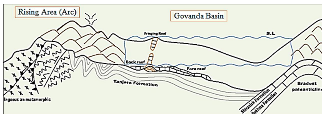
Fig.8: Depositional model of Govanda Formation during Early Miocene (Smail, 2015)
