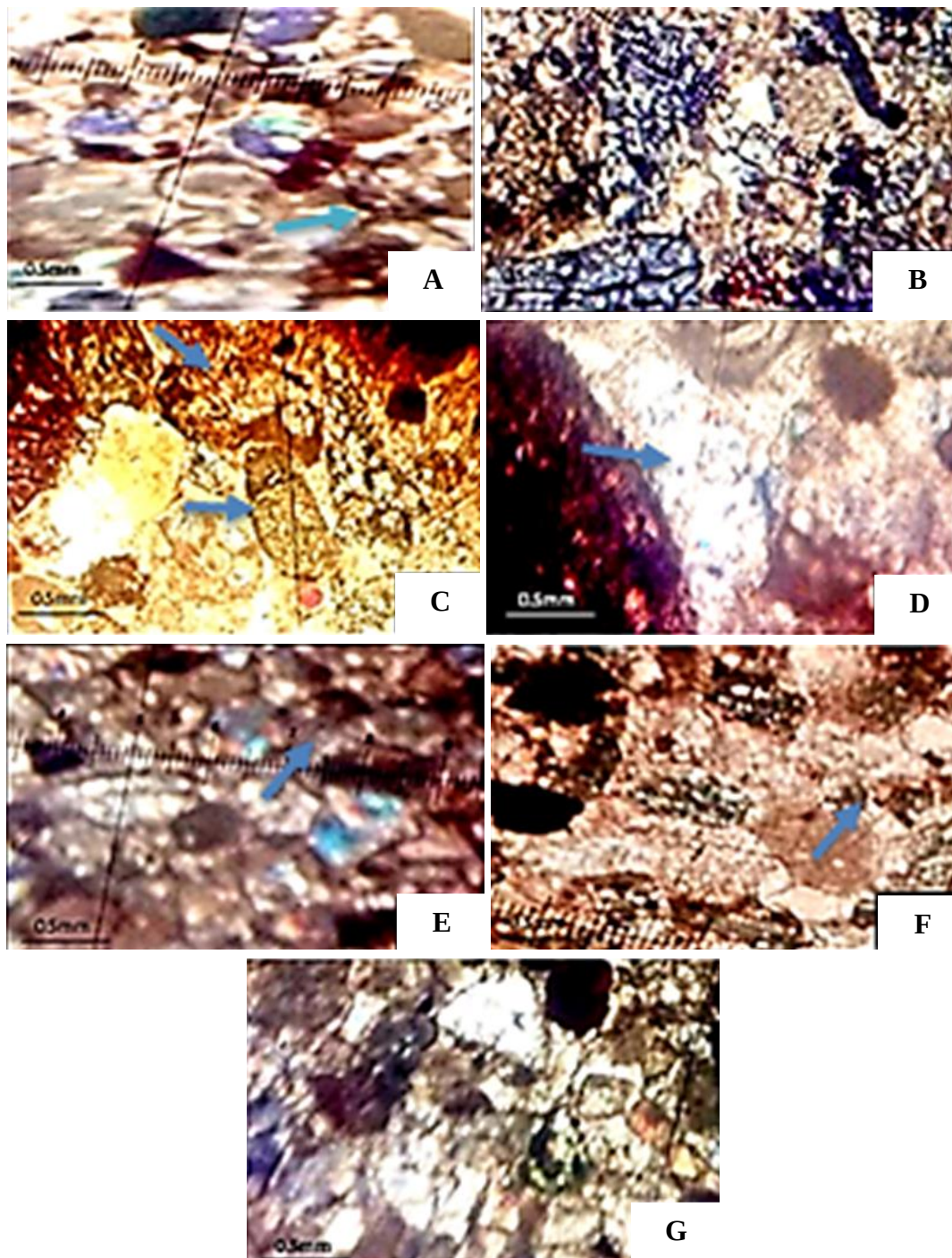
Fig.7: A) Pressure solution represented by the development of penetration between grains and solution seams (Mag.: 40X, XPL); B) Dissolution of a fossil after cementation (Mag.: 40X, XPL); C) Mechanical compaction (Mag.: 40X, XPL); D) Drusy and intergranular cement within the grains. (Mag.: 40X, XPL); E) Silicification (chertification) of skeletal grains (shells) (Mag.: 40X, XPL) F) Micritization of skeletal grains (shells) (Mag.: 40X, XPL) and G) Recrystallization of bioclasts and other grains (Mag.: 40X, XPL)
