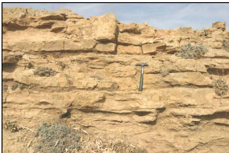
Fig.2: Limestone and dolomitic limestone of Jeribe Formation, NE limb Darzila Village (after Lawa, 2009)
