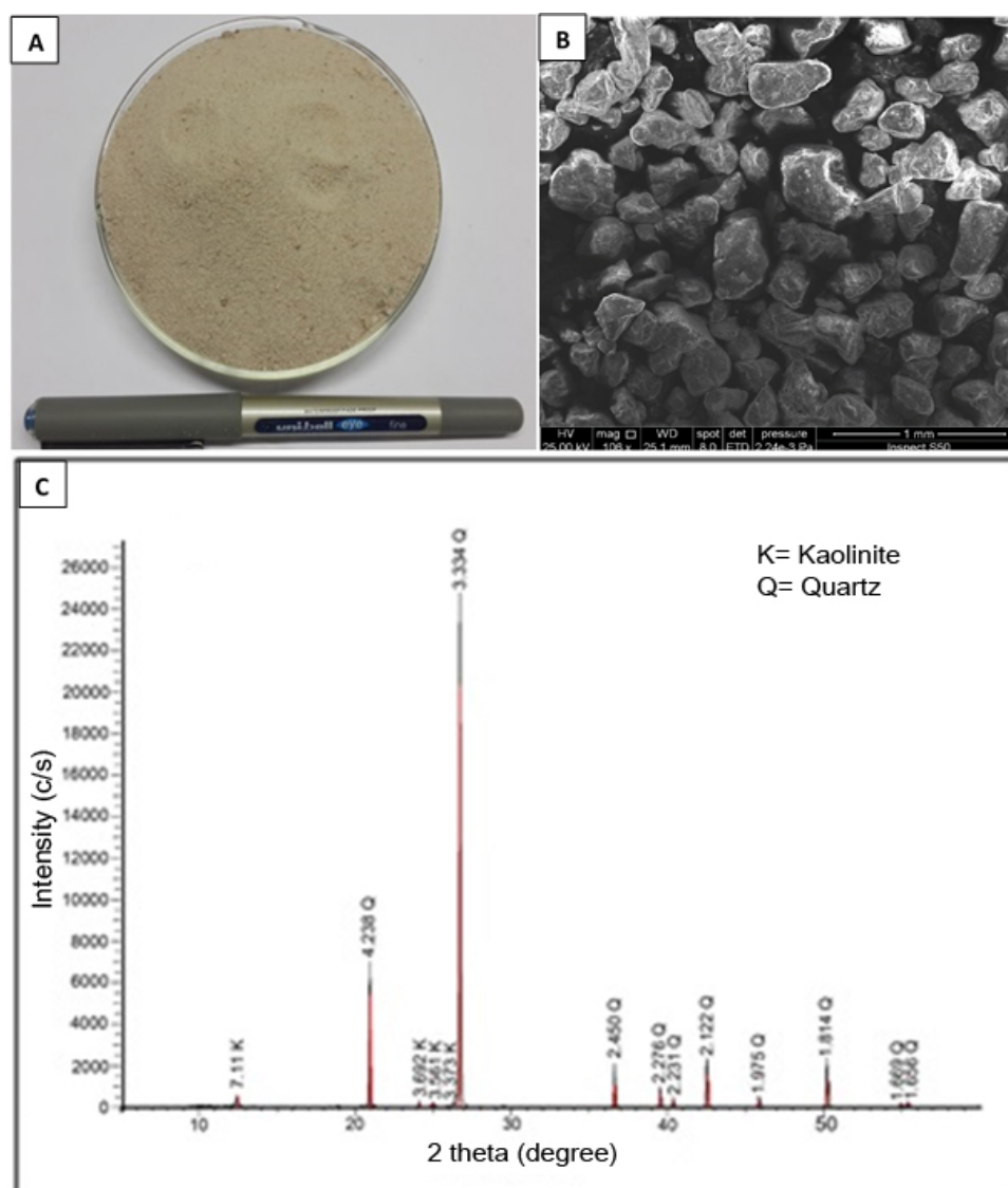
Fig.3: Silica sand sample; A) representative specimen; B) SEM image shows quartz grain; C) XRD diffractogram displays quartz as a main constituents
