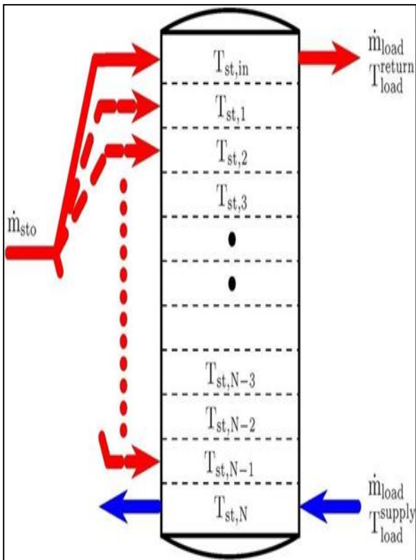
Fig. 10. Stratified Storage tank [37]
