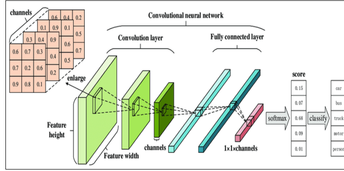
Figure 4. The architecture of CNN.
