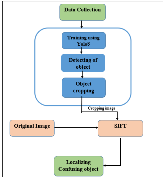
Figure 3. General block diagram of the proposed.
