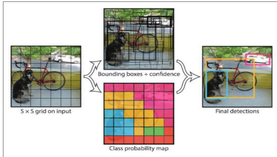
Figure 6. YOLO framework.
