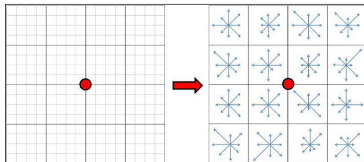
Figure 9. Key point descriptor [39].
