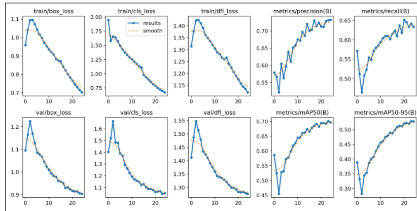
Figure 12. Trained stage for only 25 epochs.
