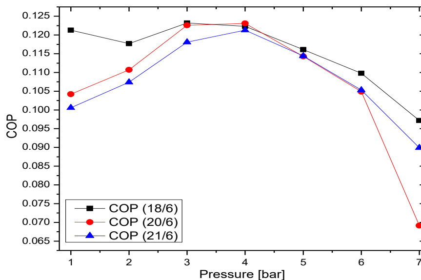
Fig. 9. Alteration of COP with pressure for three different days (18 th , 20 th , and 21 st of June-2023).
