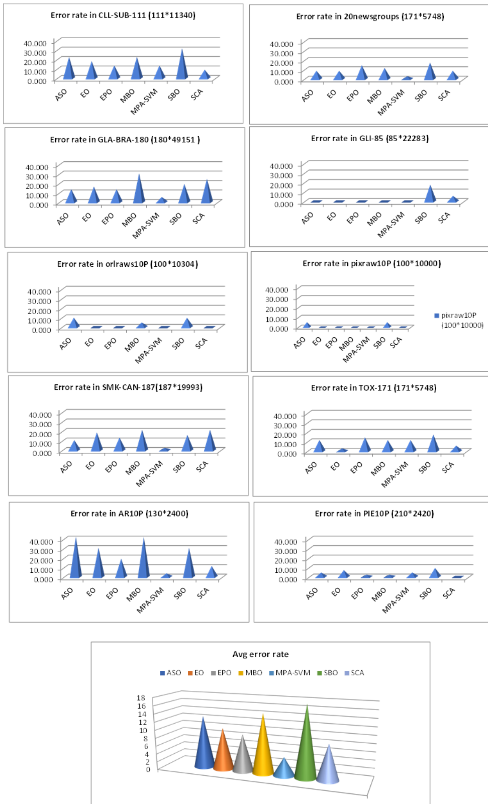
Fig .2 Comparing the suggested methods depending on the rate of classification error
