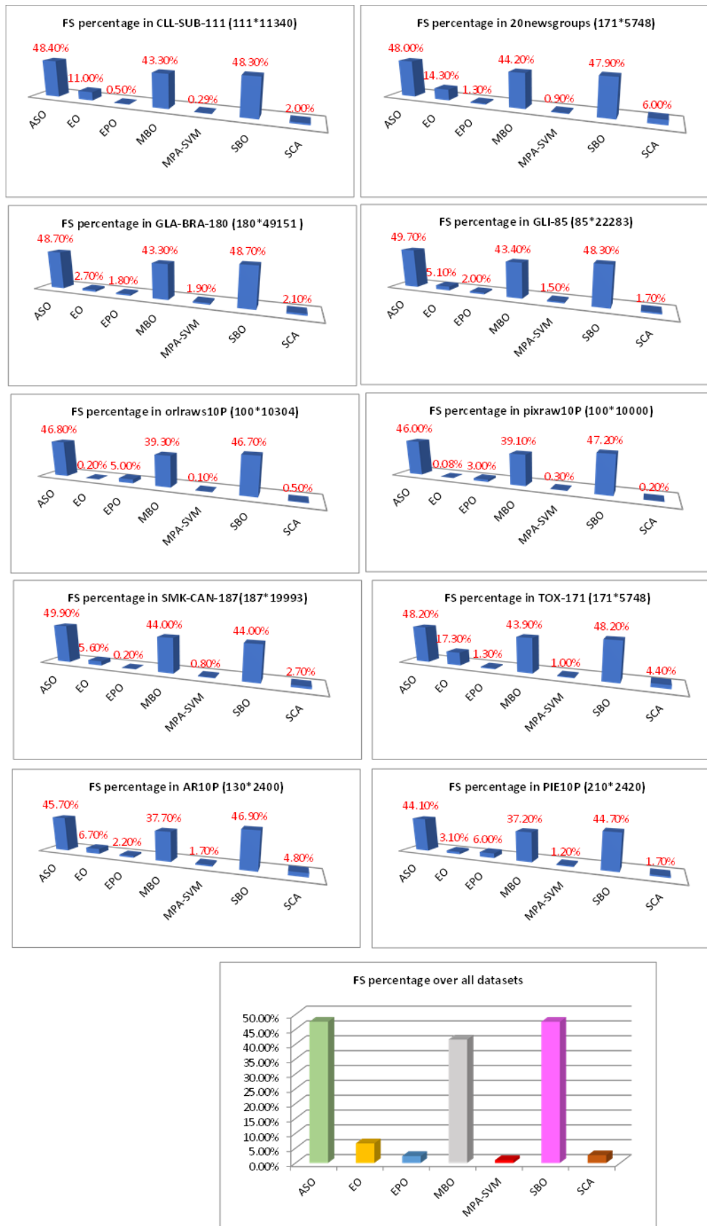
Fig. 4 Comparing the suggested methods depending on the average selected features percentage
