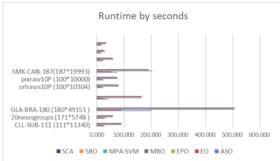
Fig. 5 Comparing the proposed MPA-SVM based on algorithms runtimes
