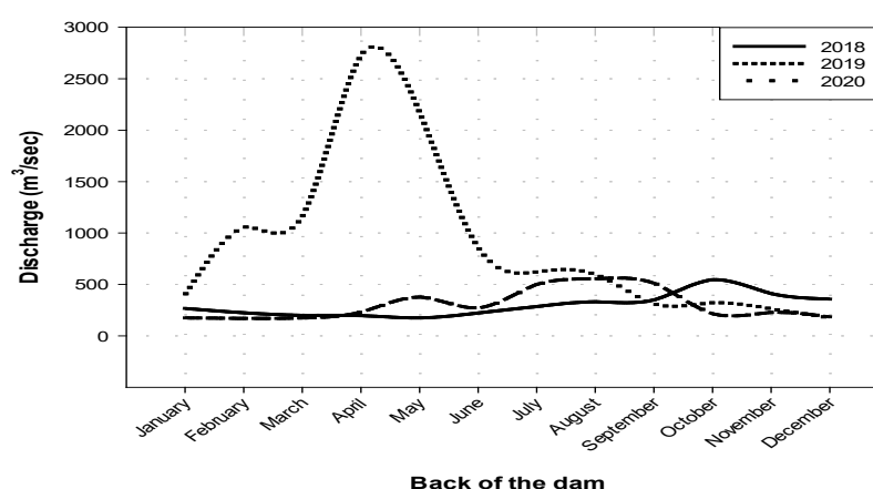
Figure 4. Discharge in the back of Mosul dam.
