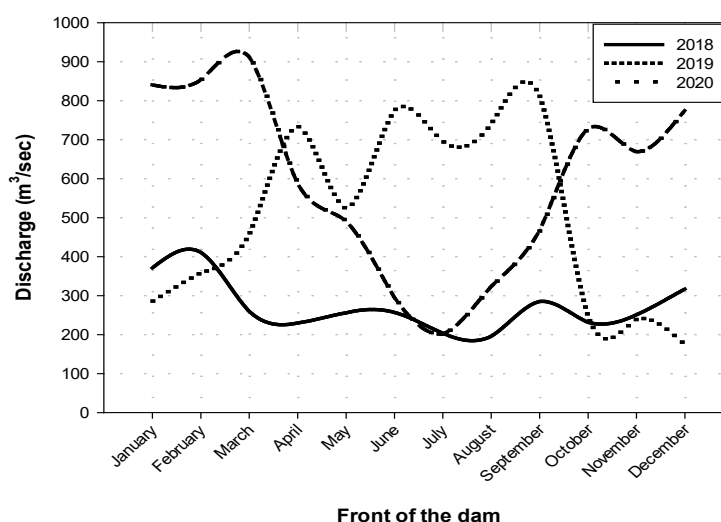
Figure 5. Discharge in the front of Fallujah dam.
