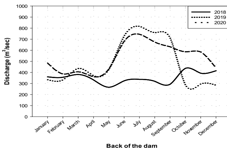
Figure 6. Discharge in the back of Fallujah dam.
