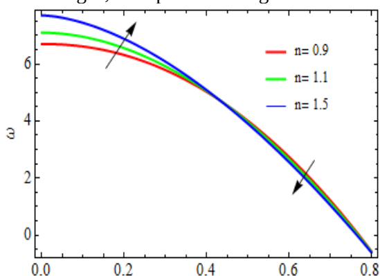
Figure 2- Effect of n on the axial velocity w at k = 0.1, b = 0.05, \phi = 0.2, F = 2, z = 0.1
