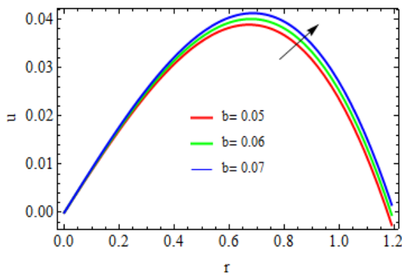
Figure 9- Effect of b on the radial velocity u at n = 1.1 , k = 0.1 , \phi = 0.2 , p = 1 , z = 2
