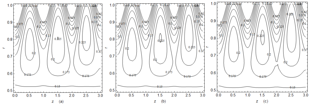
Figure 26- Effect of (a) n = 1.1 , (b) n = 1.15 , (c) n = 1.25 on the stream line at b = 0.05 , k = 0.1 , \phi = 0.2 , F = 0.2
