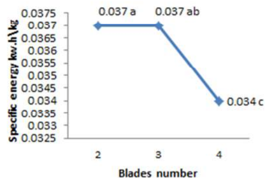
Figure 3 Effect of blade number on specific energy consumption
