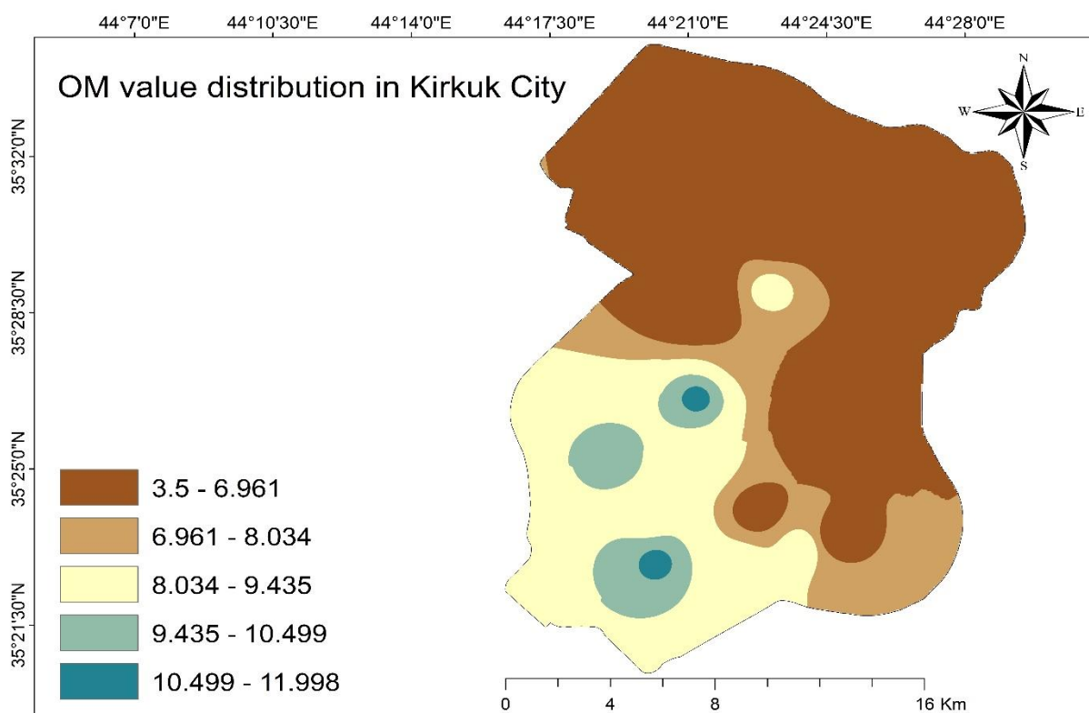
Fig. 8. Kriging representation of organic matter distribution.
