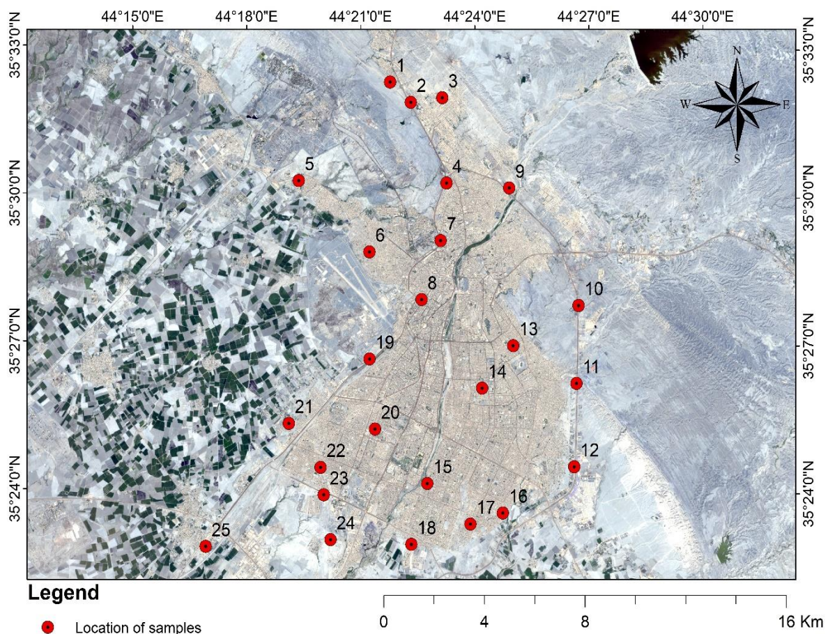
Fig. 2. Surface soil sampling locations in Kirkuk City.
