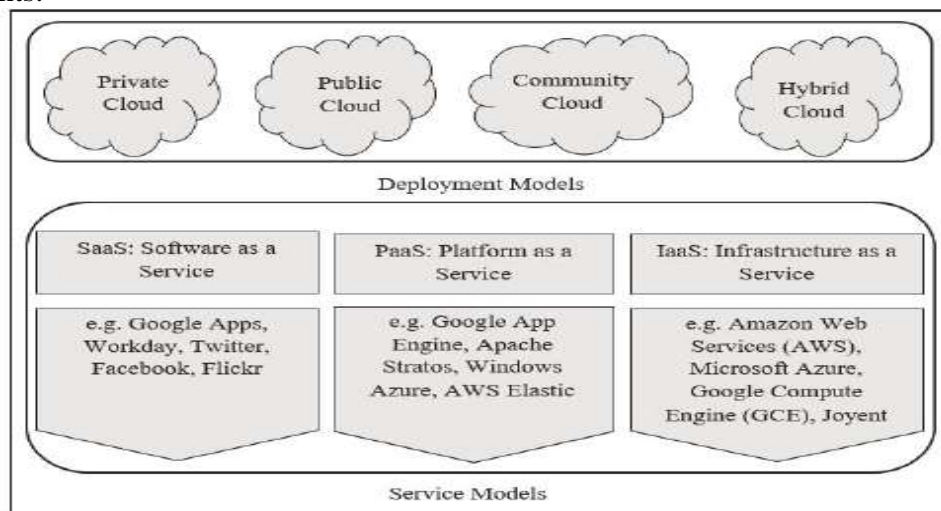
Figure 1- Cloud computing service model [4]
