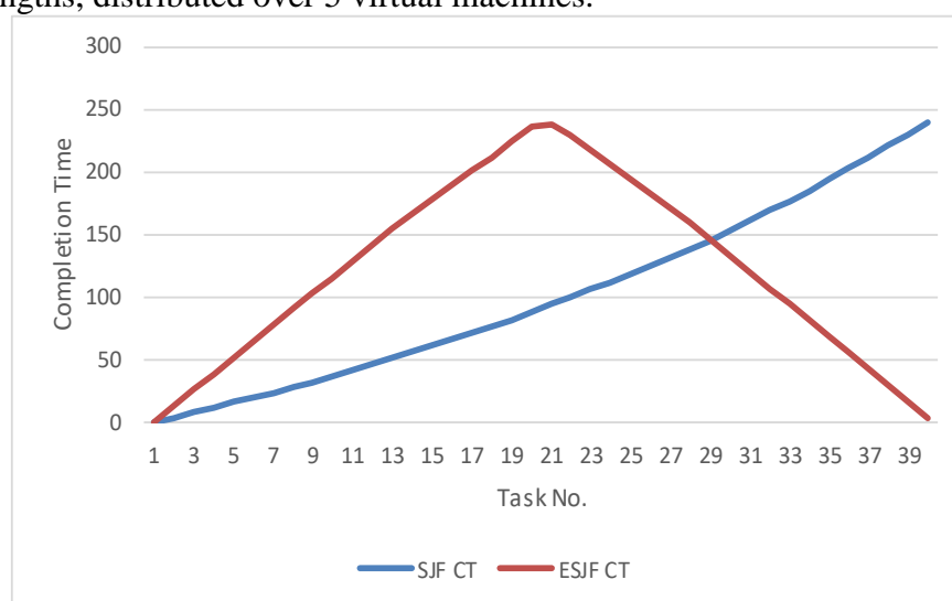
Figure 4- Comparison of completion time
