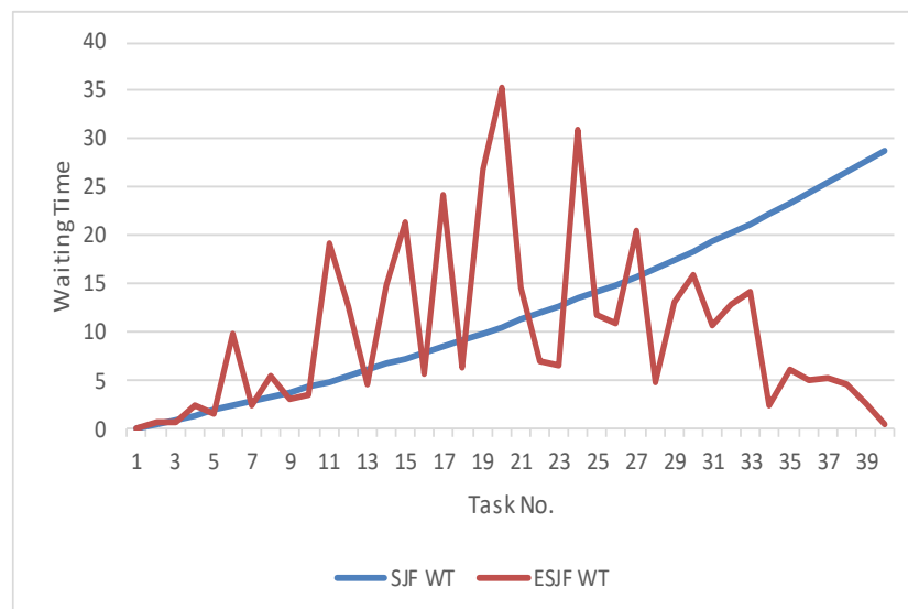
Figure 3- Comparison of waiting time
