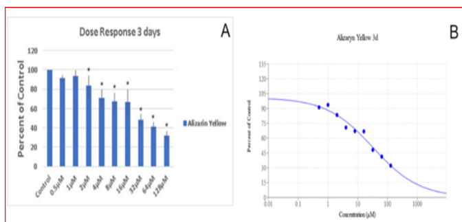
Fig – 19: Alizarin Yellow's effect on GB1B proliferation and calibration curves for IC 50 is shown in Figures A and B, respectively, after three days of treatment. In a standard medium, 5 10 4 cells/well of cells were seeded. MTT assay has been utilized to assess the cytotoxic effects of Alizarin Yellow three days after treatment with increasing drug concentrations. Results are given as percentages compared to the control. The data shows the average and standard deviation across three different experiments. The error bars represent the linear model fit into data, that is the mean SD with each drug condensation. * Denotes a significant deviation from the control (p 0.05).
