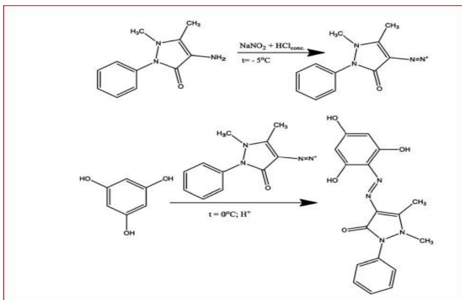
Scheme -18: Synthesis steps of \text{H}_3\text{L}_1 .
