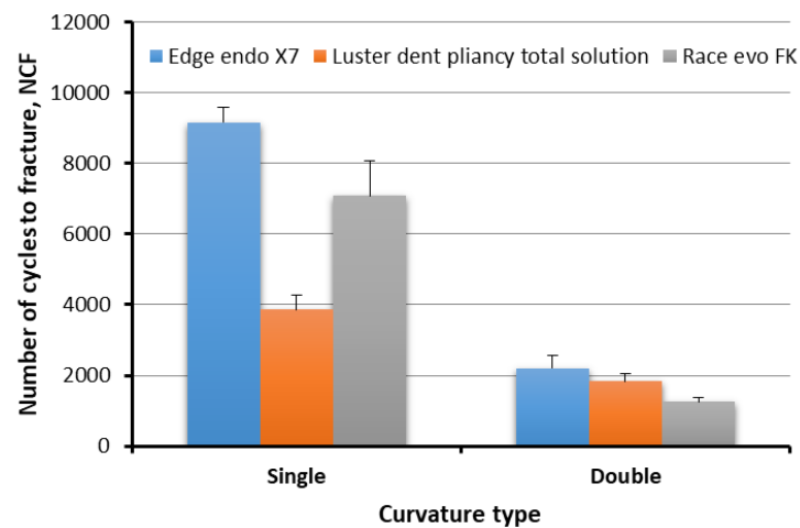
Figure 3: Bar chart showing the mean and standard deviation of the number of cycles to fracture (NCF) for the groups
