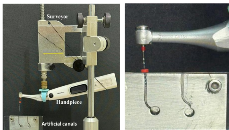
Figure 2: (a) Dental handpiece mounted on a surveyor with a file positioned inside the block; (b) magnified view of the artificial canal.
