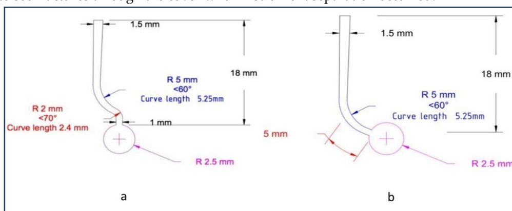
Figure 1: (a) Double curved artificial canal and (b) single curved artificial canal (adapted from (1) )
