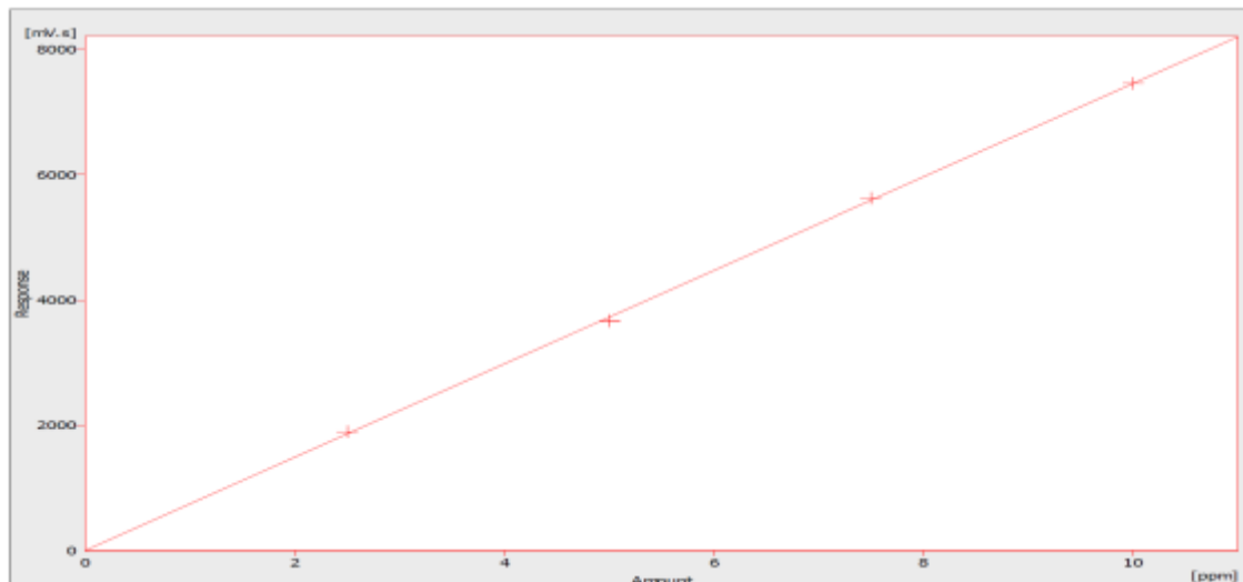
Figure 1. Calibration curve of pemetrexed by HPLC-UV
