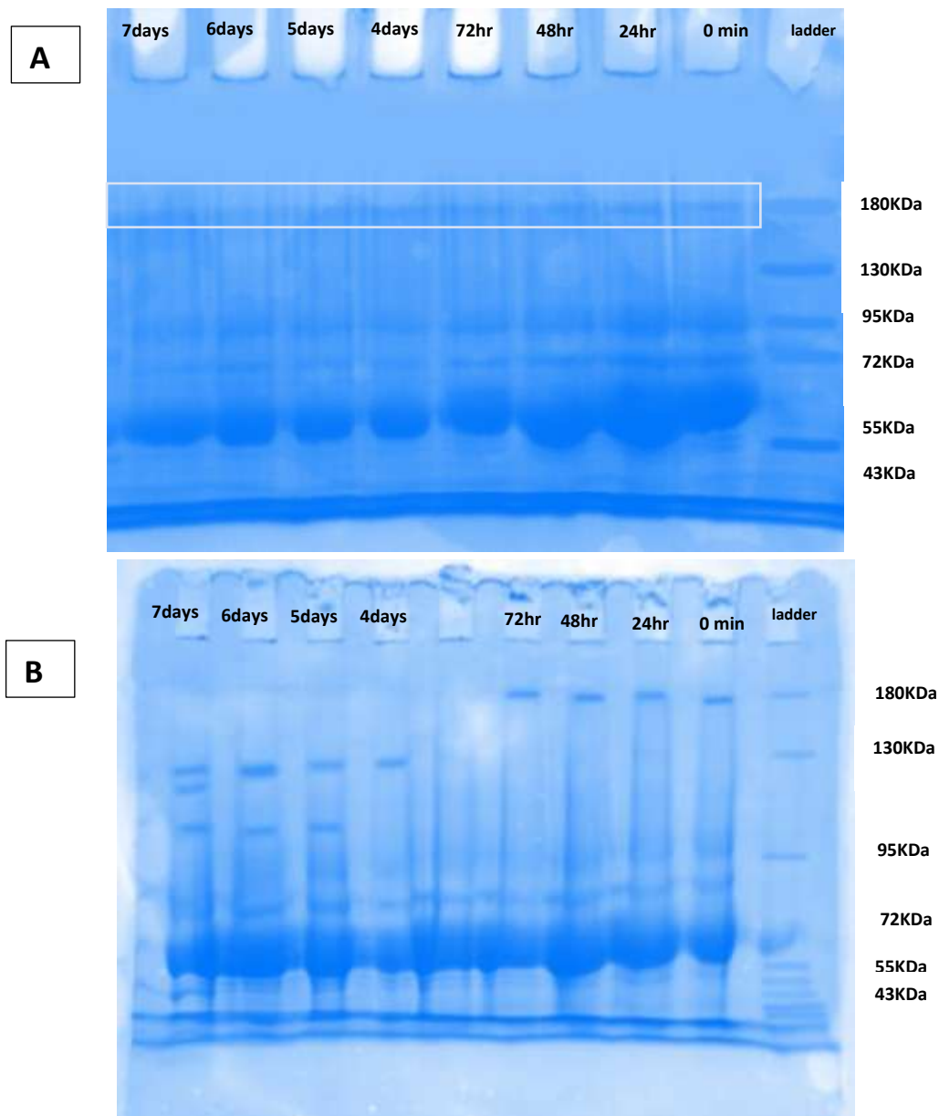
Figure 3. Stability of Pem-AtZ conjugate in human plasma by SDS- PAGE electrophoresis: (A) AtZ-PEG-Pem conjugate and (B) AtZ-GABA-Pem conjugate in which, Lane1(Ladder) Lane2(the conjugate at 0 min before storage) Lane3(conjugate at 24h) Lane4(conjugate at 48h) Lane5(conjugate at 72h) Lane6(conjugate at 4 days) Lane7(conjugate at 5 days) Lane8(conjugate at 6 days) Lane 9 (conjugate at 7 days).
