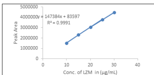
Figure 7 Calibration curve for LZM
