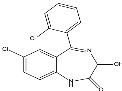
Figure 1 Structural formula of lorazepam
