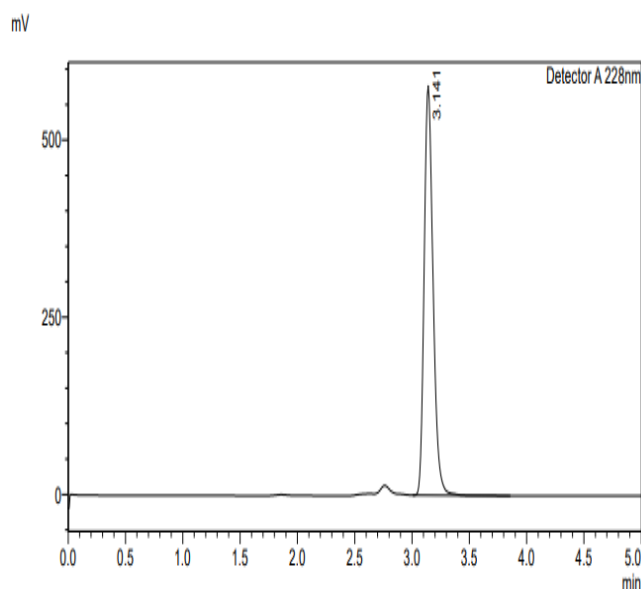
Figure 3 Chromatogram of the L3 column pH Effect
