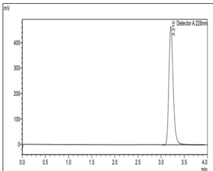
Figure 5 Chromatogram of LZM at 30°C
