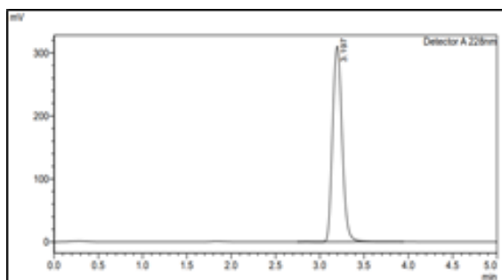
Figure 9 Chromatogram of LZM drug at a concentration of 15 \mu\text{g/ml}
