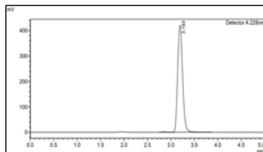
Figure 10 Chromatogram of LZM at a concentration of 20 \mu\text{g/ml}
