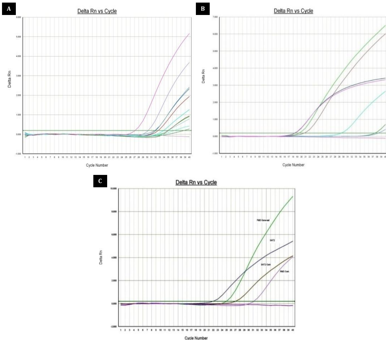
Figure 1. Amplification plots from RT-qPCR showing the detection of FMDV-specific genes. (A) Amplification curve for the 3D gene from prepared clinical samples, indicating general FMDV positivity. (B) Amplification curve for the 1D gene from prepared clinical samples, confirming the presence of the SAT2 serotype. (C) Amplification curves for both the 1D and 3D genes from tissue culture samples, demonstrating successful virus isolation and propagation, with 1D confirming SAT2 specificity and 3D indicating general FMDV detection
