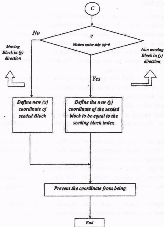
Fig. (2) Flowchart for tracing forward motion
