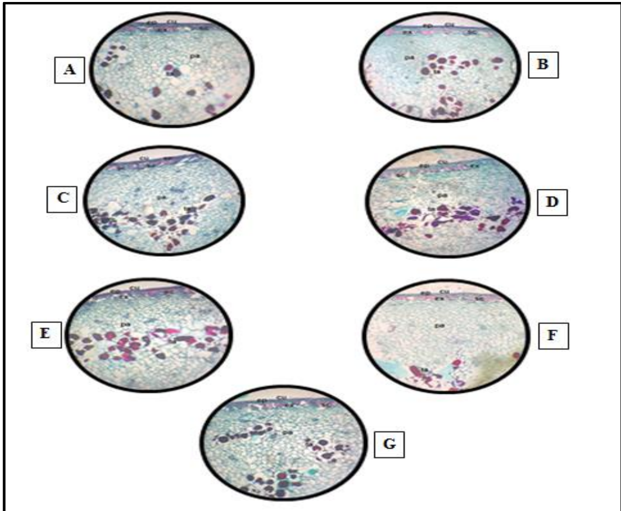
Figure 1: Effect of different concentrations of pollen extract and gibberellic acid on some anatomic characteristics. A: 30gL -1 pollen extract treatment; B: Control treatment; C: 60gL -1 pollen extract treatment; D: 25mgL -1 GA 3 treatment; E: 50mgL -1 GA 3 treatment; F: 75mgL -1 GA 3 treatment; G: 100mgL -1 GA 3 treatment.
