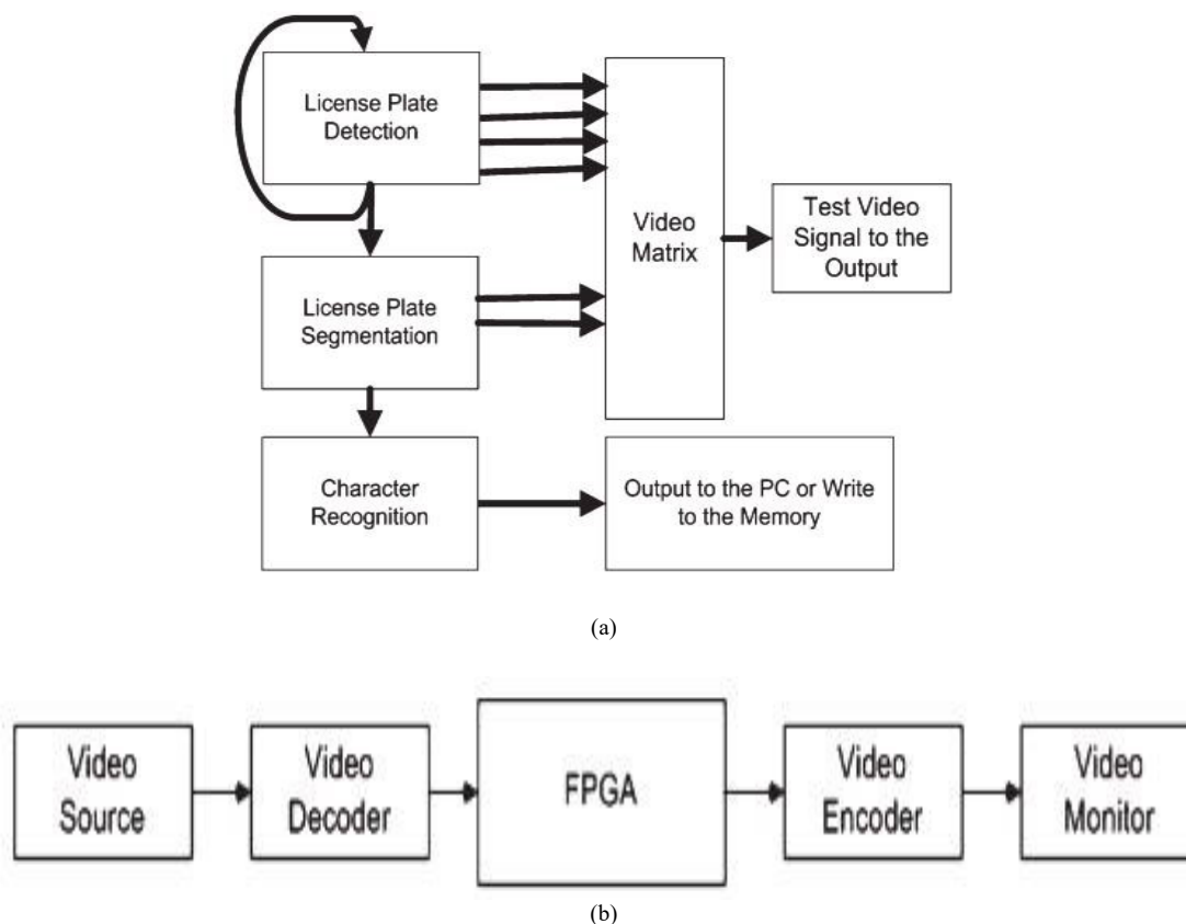
Fig.15. a) Embedded LPR system block diagram, b) Hardware block diagram [22]
