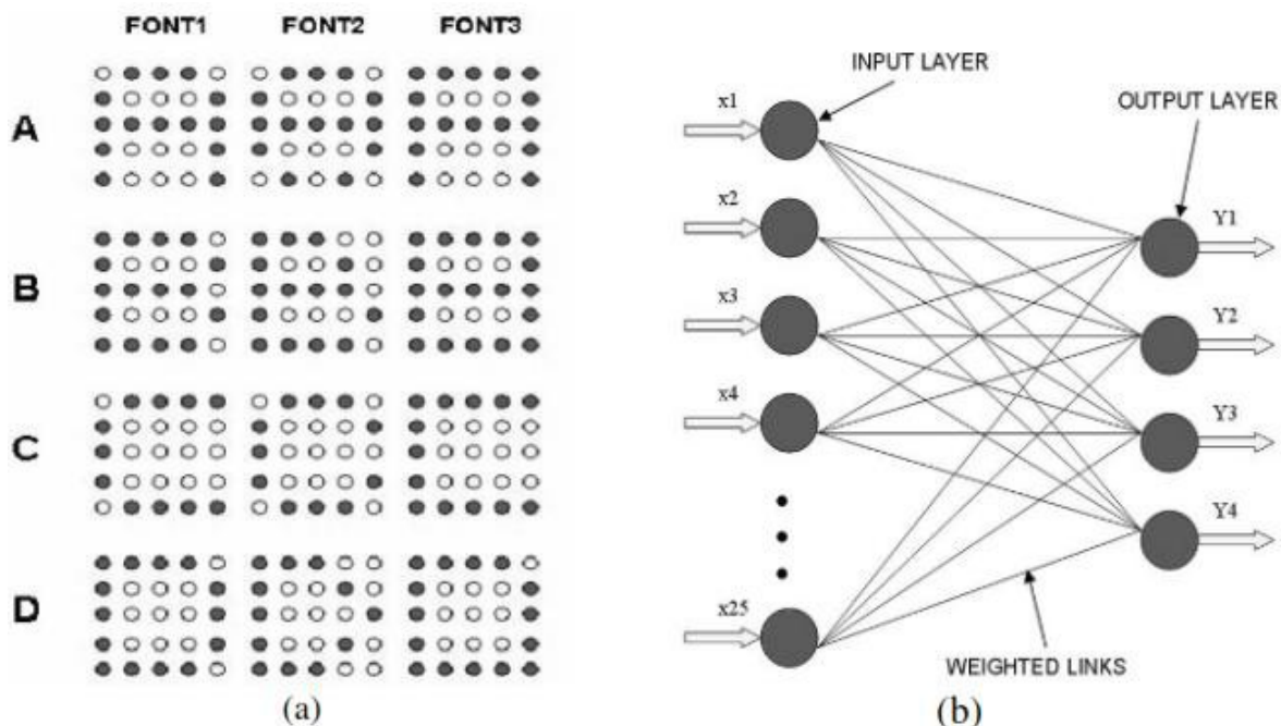
Fig.10. (a) Patterns of input with three distinct fonts for every character. (b) Used Perceptron model for character recognition issue[18].
