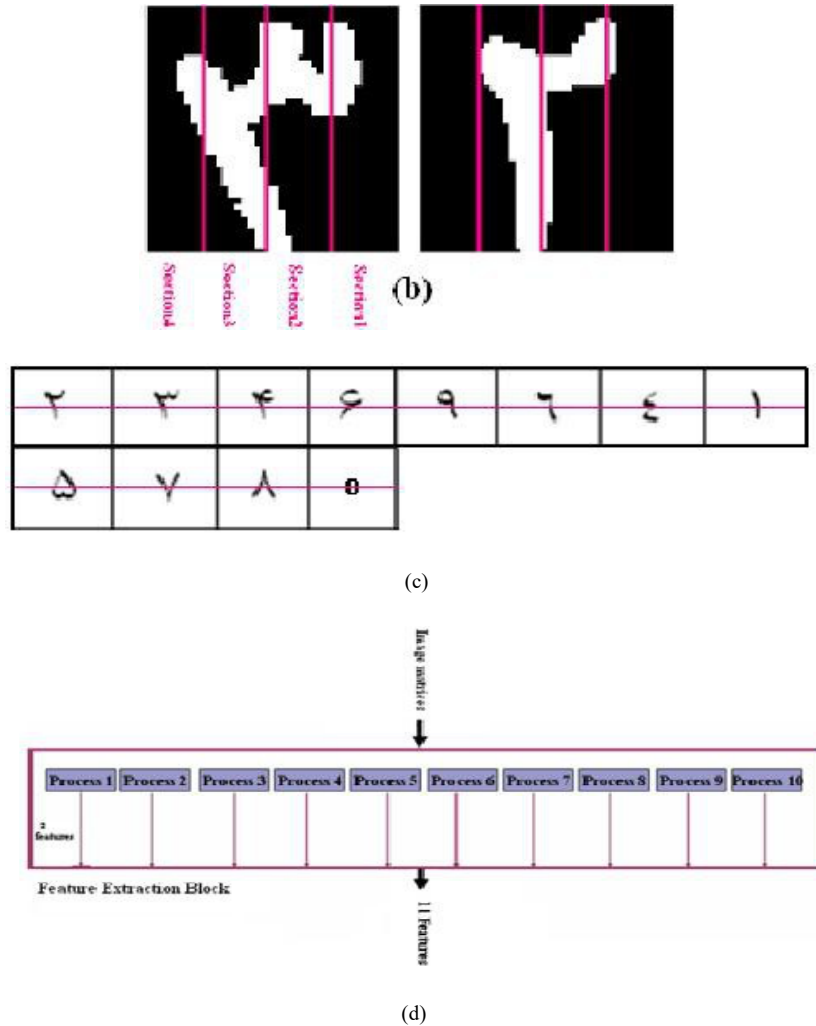
Fig.16. (a) & (b) Pictures are divided to four horizontal and four vertical sections, (c) Count the number of intersections along horizontal ray of and written and typed images, (d) The block diagram of feature extraction block [19]
