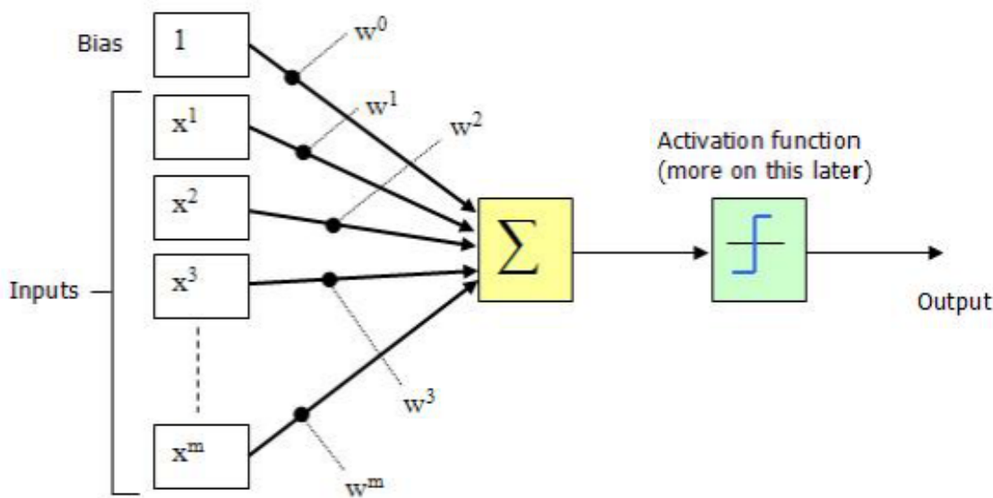
Fig.7. An Artificial Neuron
