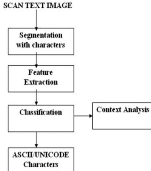
Fig.14. Stages in OCR Design [20]
