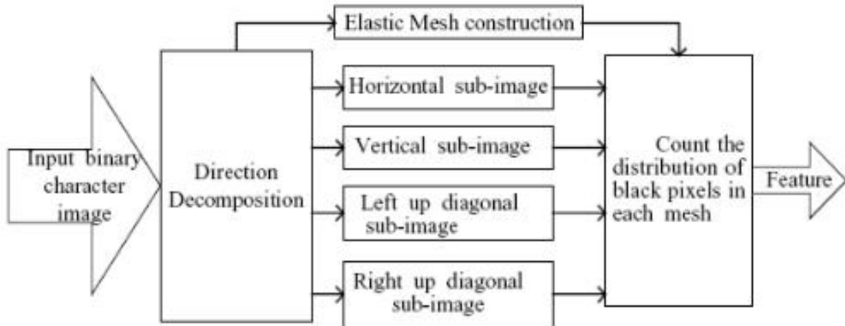
Fig.13. The block diagram of elastic meshing directional feature extraction (Moradi et al., 2009)
