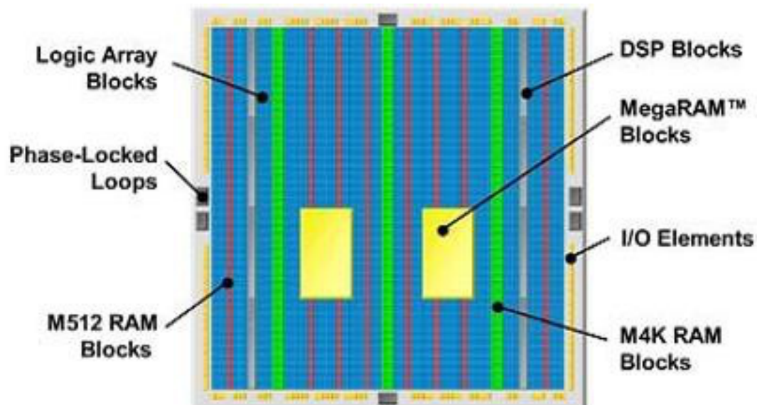
Fig. 9. Altera FPGA Structure
