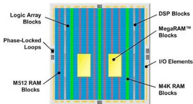
Fig.1. Altera FPGA Structure
