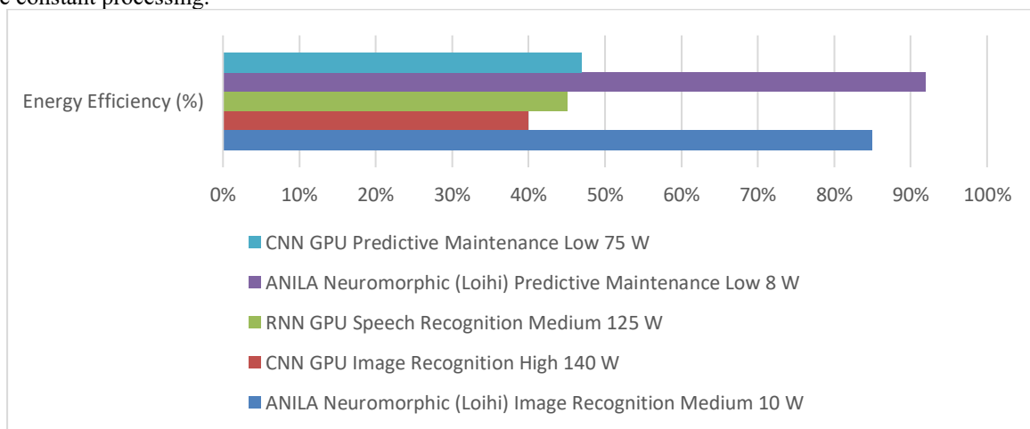
Fig. 2. Energy Efficiency Comparison Across Different Workloads for ANILA, CNN, and RNN.
