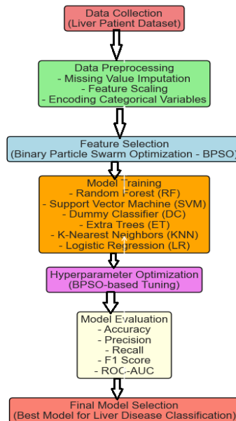
Fig. 6. The proposed framework.
