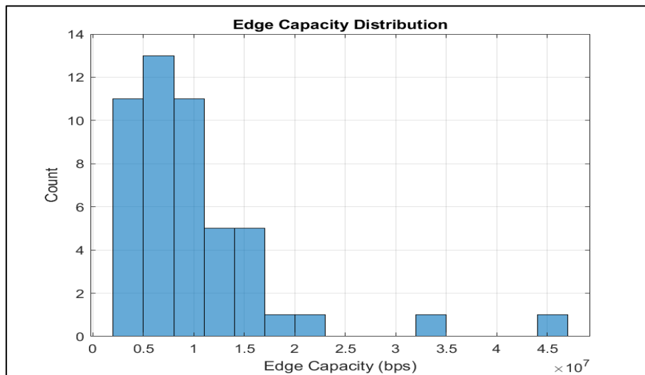
Fig. 8. Edge Capacity Histogram
