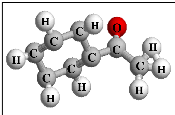
Fig(1) Geometry optimization of Acetophenone
