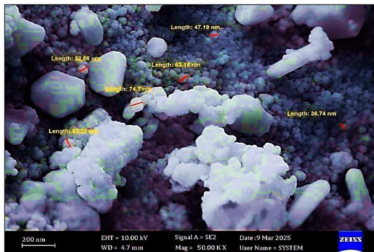
Figure 4. FESEM pictures of the Mn_3O_4:Ag nanocomposite
