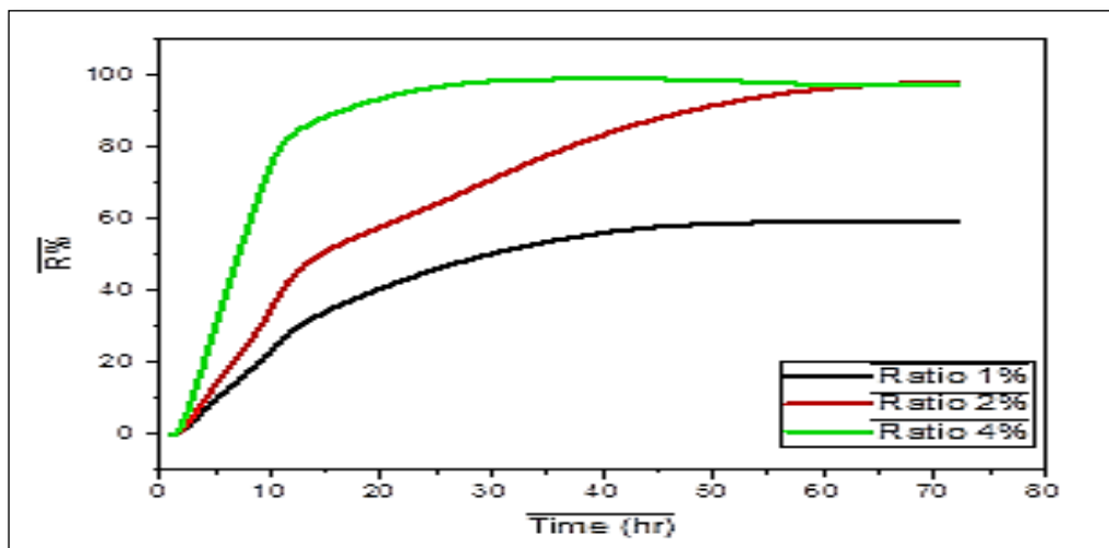
Figure 5. The R% of MB using coated films with Mn_3O_4:Ag -coated films (1, 2, and 4)%
