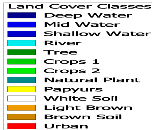
Figure 3. Land cover after classification based on training samples "EPSG:32638-WGS84/UTM Zone 38"
