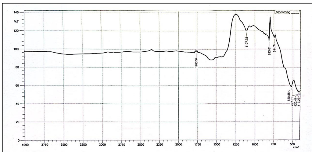
Figure 3. FT-IR analysis of the \alpha - Fe_2O_3 nanomaterial produced by treating the plant extract with the inorganic substance potassium hexacyanoferrate (III) K_3[Fe(CN)_6] after carrying out all preparation methods
