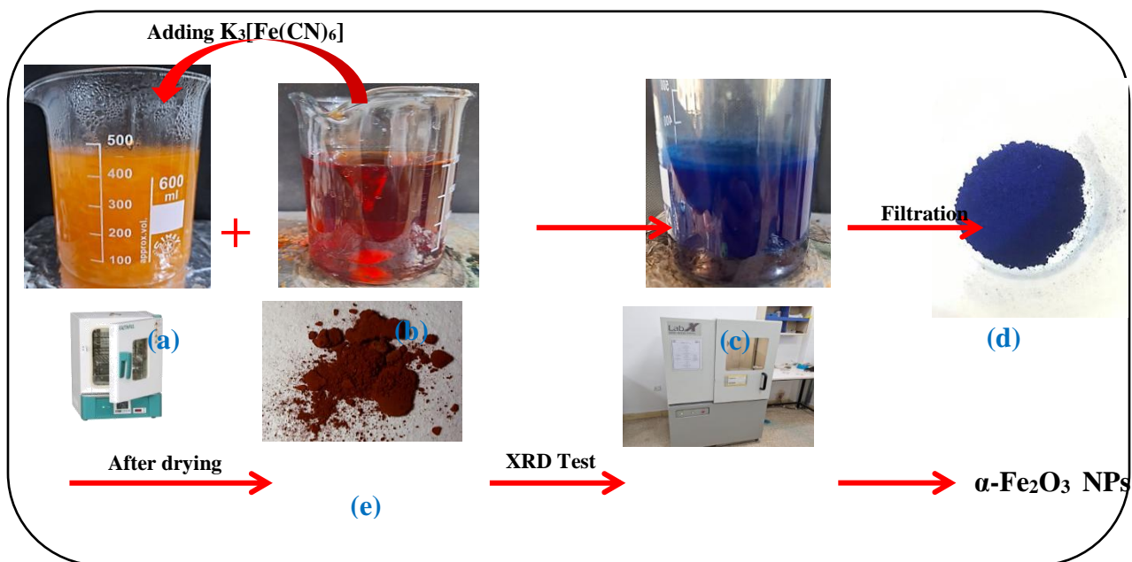
Figure 1. The method for preparing \alpha-Fe_2O_3 NPs involves the main steps from the plant extract to drying the NPs: (a) plant extract, (b) solution of potassium hexacyanoferrate, (c) mix a+b, (d) powder of \alpha-Fe_2O_3 NPs before drying, (e) powder of \alpha-Fe_2O_3 NPs after drying.
