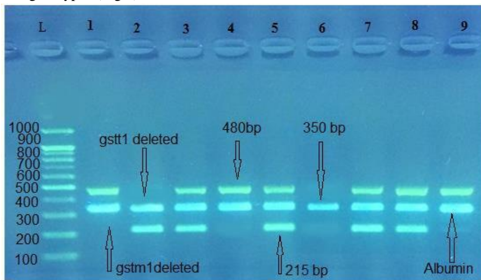
Fig (1) : Electrophoresis of PCR products on agarose gel 1% ( 100 volt / 1 hr ) . All samples belong to patients. Lane 1,4,9 : gstm1 deletion , Lane 2 : gstt1 deletion , Lane 3 ,5,7,8 : Normal genotype, Lane 6 : Null genotype, Lane L : DNA ladder ( 100 -1000 bp).
