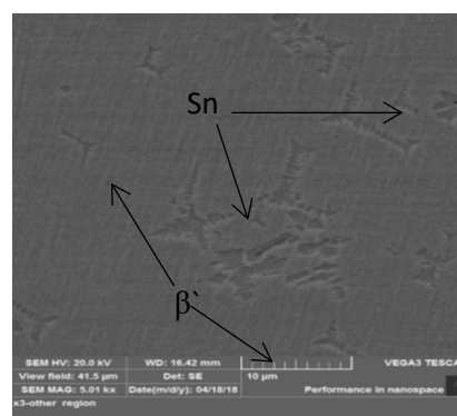
Figure 6: The (S1) alloy microstructure
