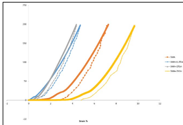
Figure 15: Thermo-Mechanical Stress –Strain Diagram.
