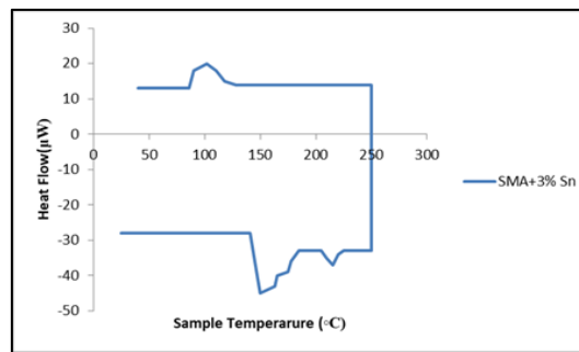
Figure 13: Thermogram of (S3) SMA.
