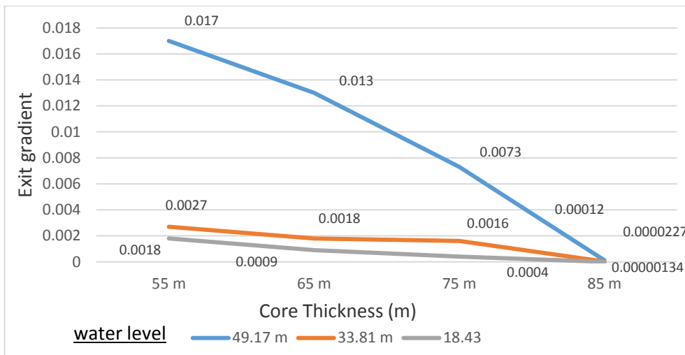
Figure 8: Relationship between exit gradient and core thickness
