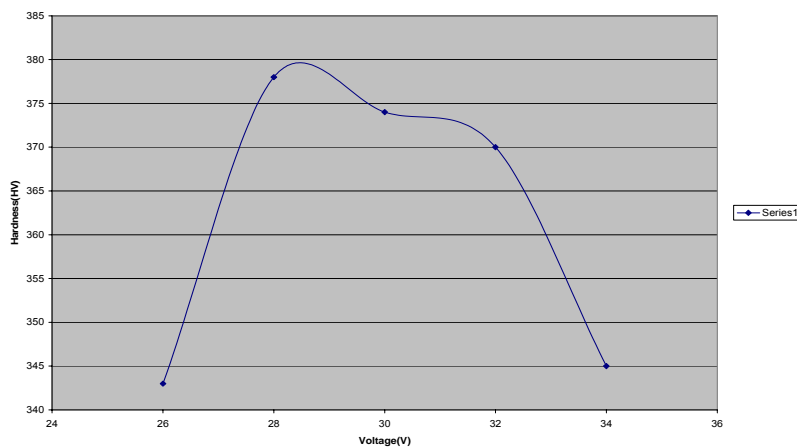
Fig (2) The relationship between the applied voltage and Hardness. Coating thickness=1.5mm.Spraying distance=13cm.
