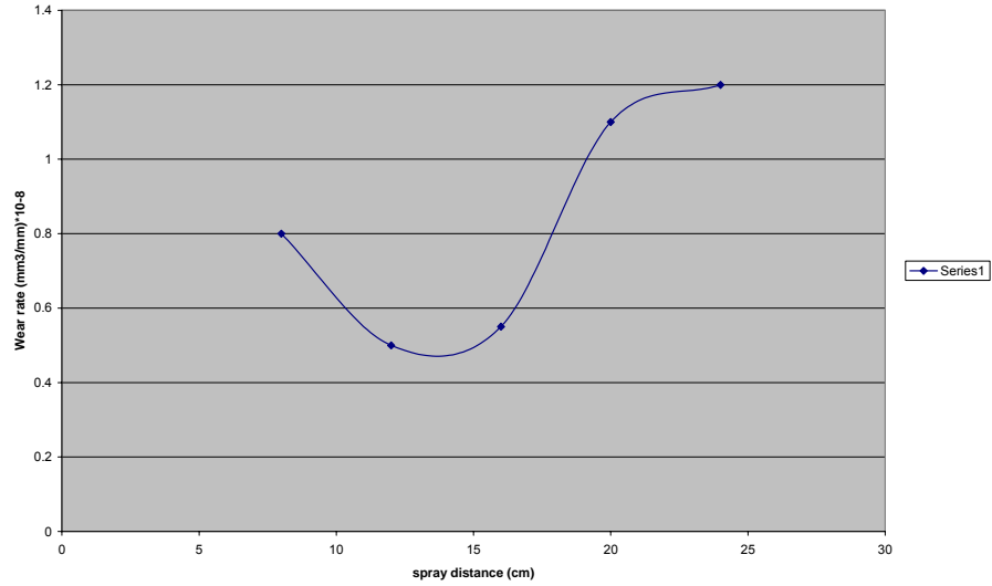
Fig (8) The relationship between the spraying distance and wear rate.
