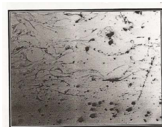
Fig. (12): Optical microscopy picture, (100X), shows the microstructure of the base with the coating layer, unetched.
