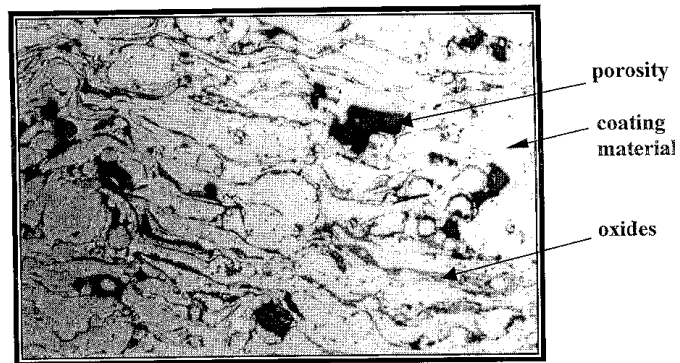
Fig (10): A typical microstructure of a sprayed coating showing the lamellar structure, oxides and porosity, (100X) unetched.
