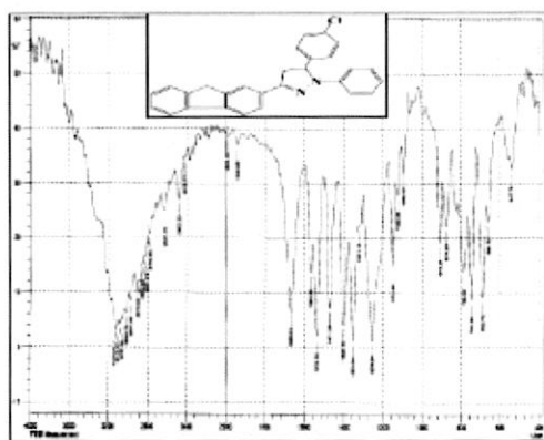
Fig.(3): FT-IR spectrum for compound (3b)
