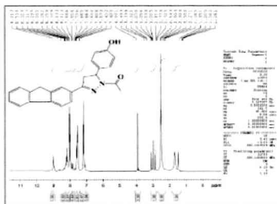
Fig.(2): 1 H-NMR spectrum for compound (2e)
