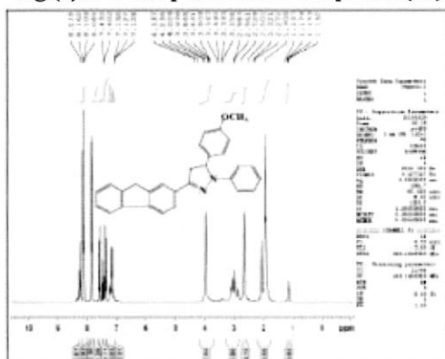
Fig.(4): 1 H-NMR spectrum for compound (3d)
