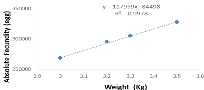
Figure 2. Relationship between female body weight and absolute fecundity in Ovaprim treated fish.
