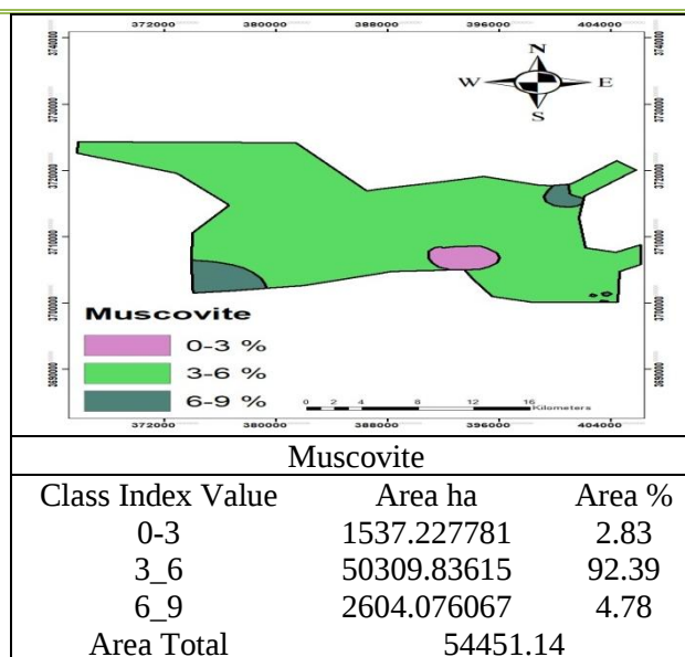
Figure 9. Spatial map of Muscovite mineral
