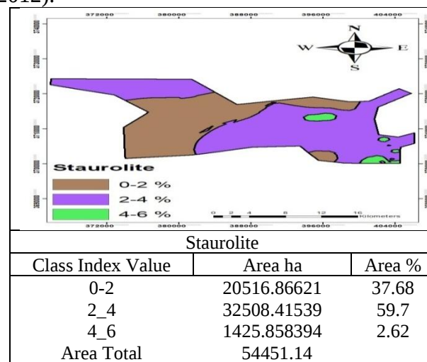
Figure12. Spatial map of Staurolite mineral
