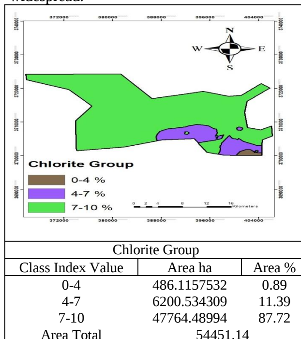
Figure 3. Spatial map of chlorite mineral
