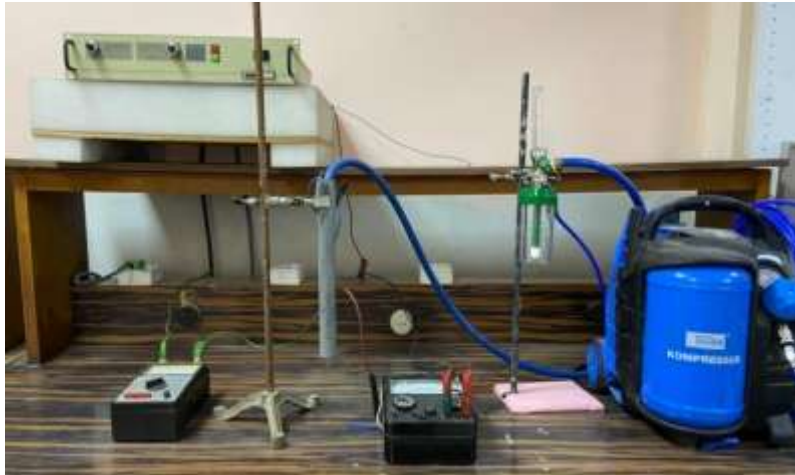
Fig. 2: A photograph the experimental setup of plasma jet systems
