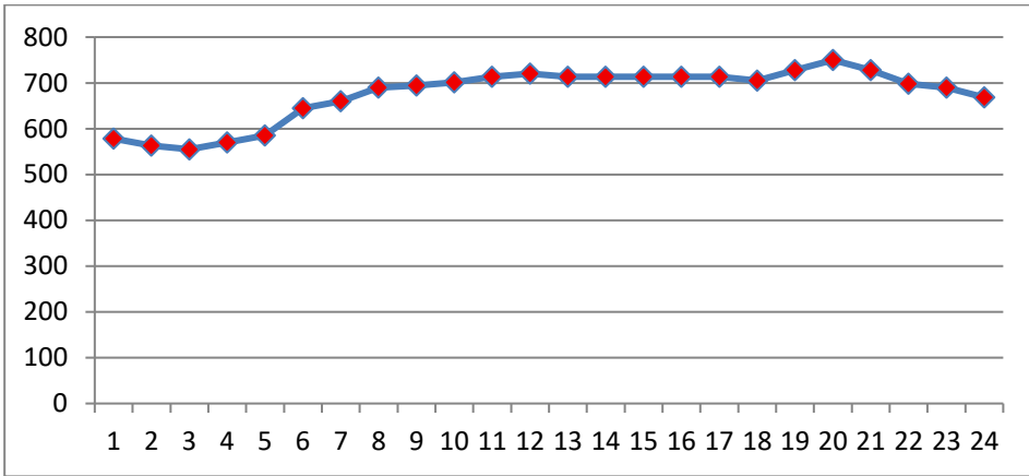
Figure (4): Electricity Consumption During the 24 Hours of the Day in Al-Anbar Governorate on 15-04-2024
