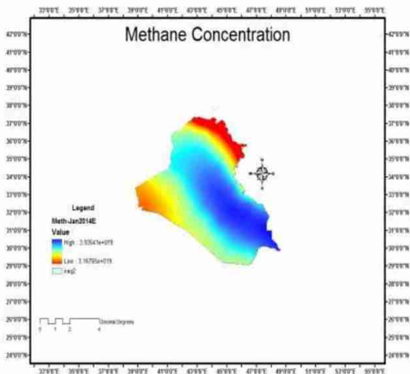
Figure (١٠): Methane map January ٢٠١٤.
