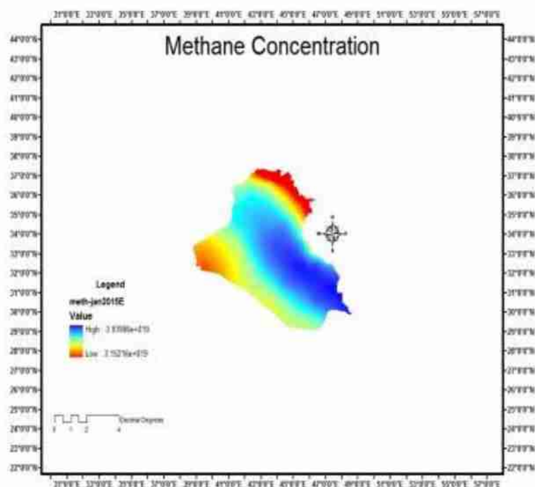
Figure (١٣): Methane map January ٢٠١٥.
