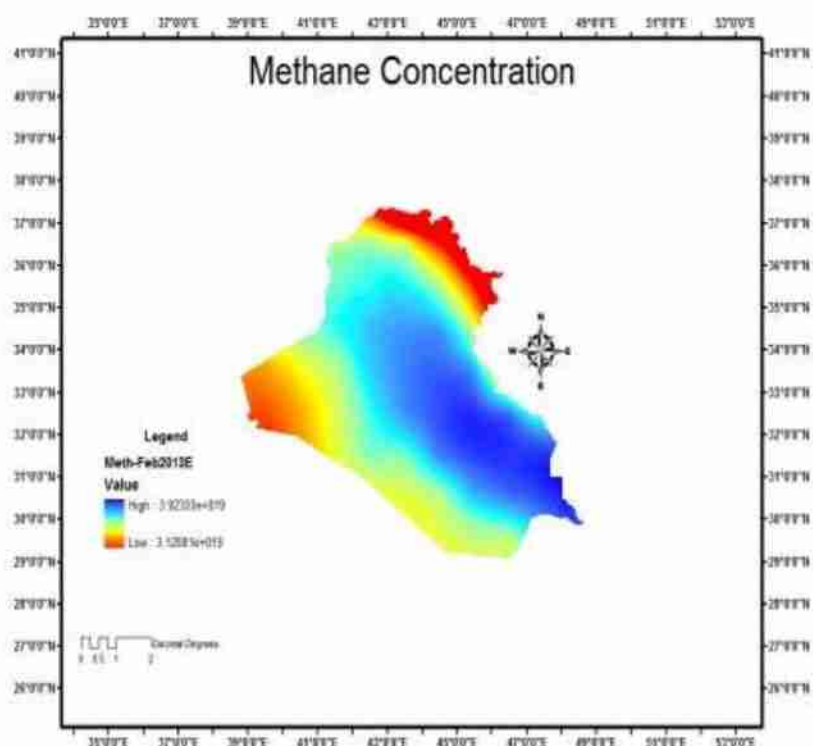
Figure (A): Methane map February ٢٠١٣.
