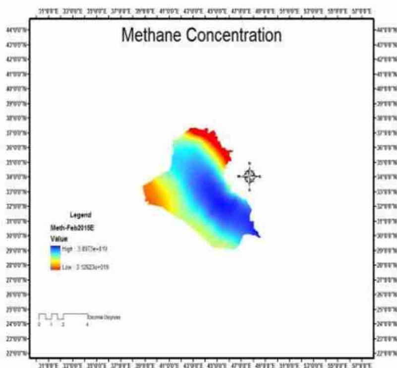
Figure (١٤): Methane map February ٢٠١٥.
