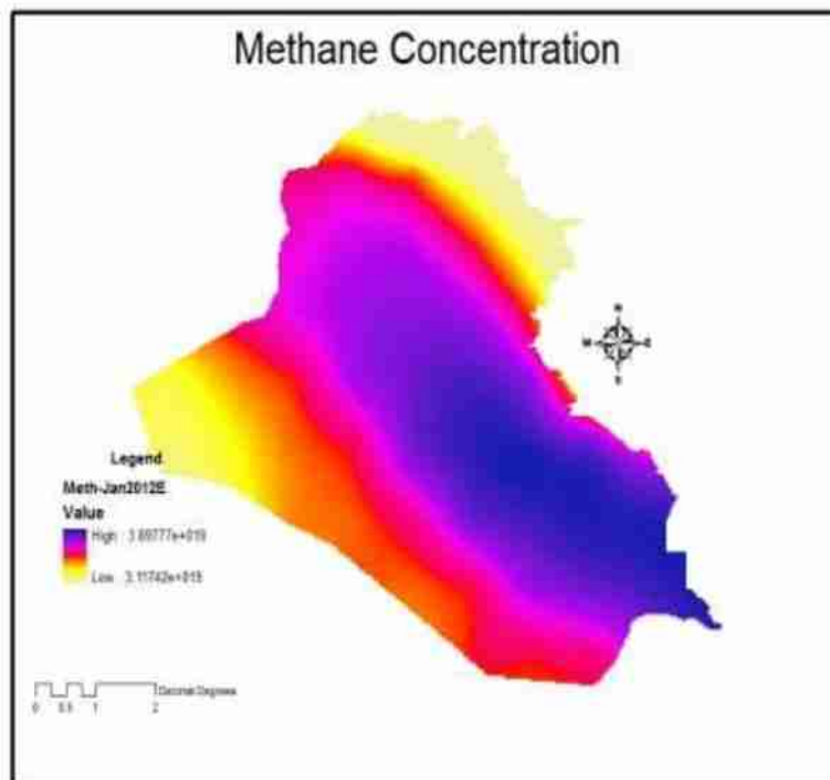
Figure (4): Methane map January 2012.
