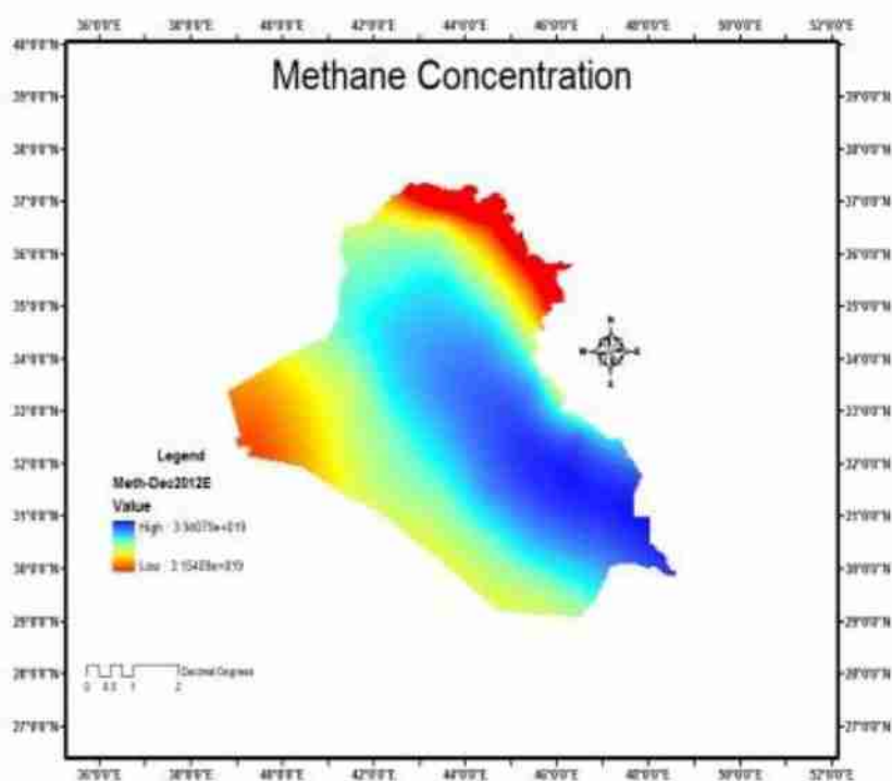
Figure (٦): Methane map December ٢٠١٢.
