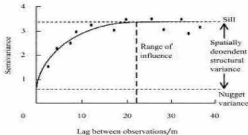
Figure (7): The variogram.
