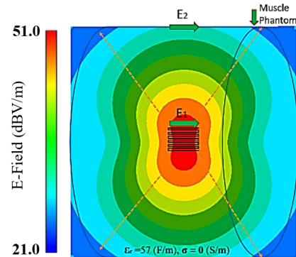
(a) Model with \epsilon_r = 57 (F/m), \sigma = 0 (S/m)
