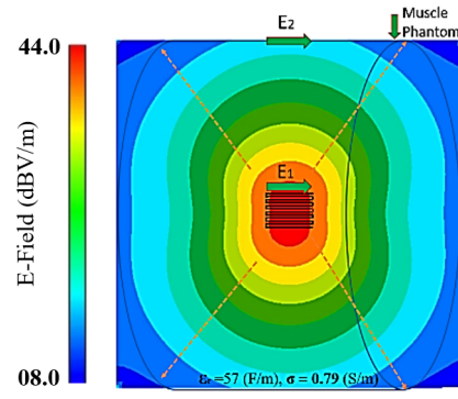
(b) Model with \epsilon_r = 57 (F/m), \sigma = 0.79 (S/m)
