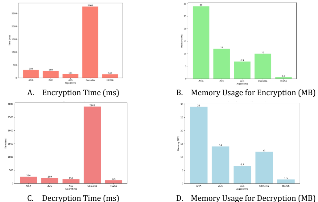
Figure 4. Performance Metrics of Cryptographic Algorithms for MP3 Processing
