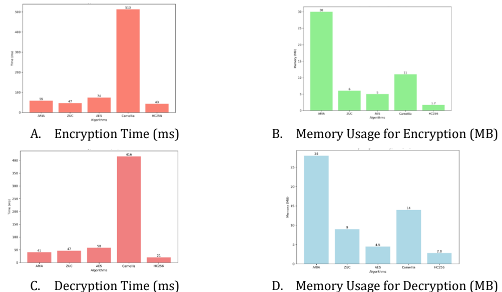
Figure 6. Performance Metrics of Cryptographic Algorithms for PDF File Processing
