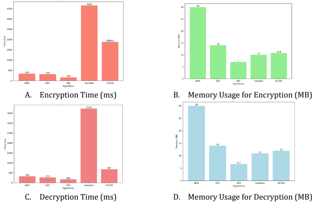
Figure 3. Performance Metrics of Cryptographic Algorithms for Image Processing
